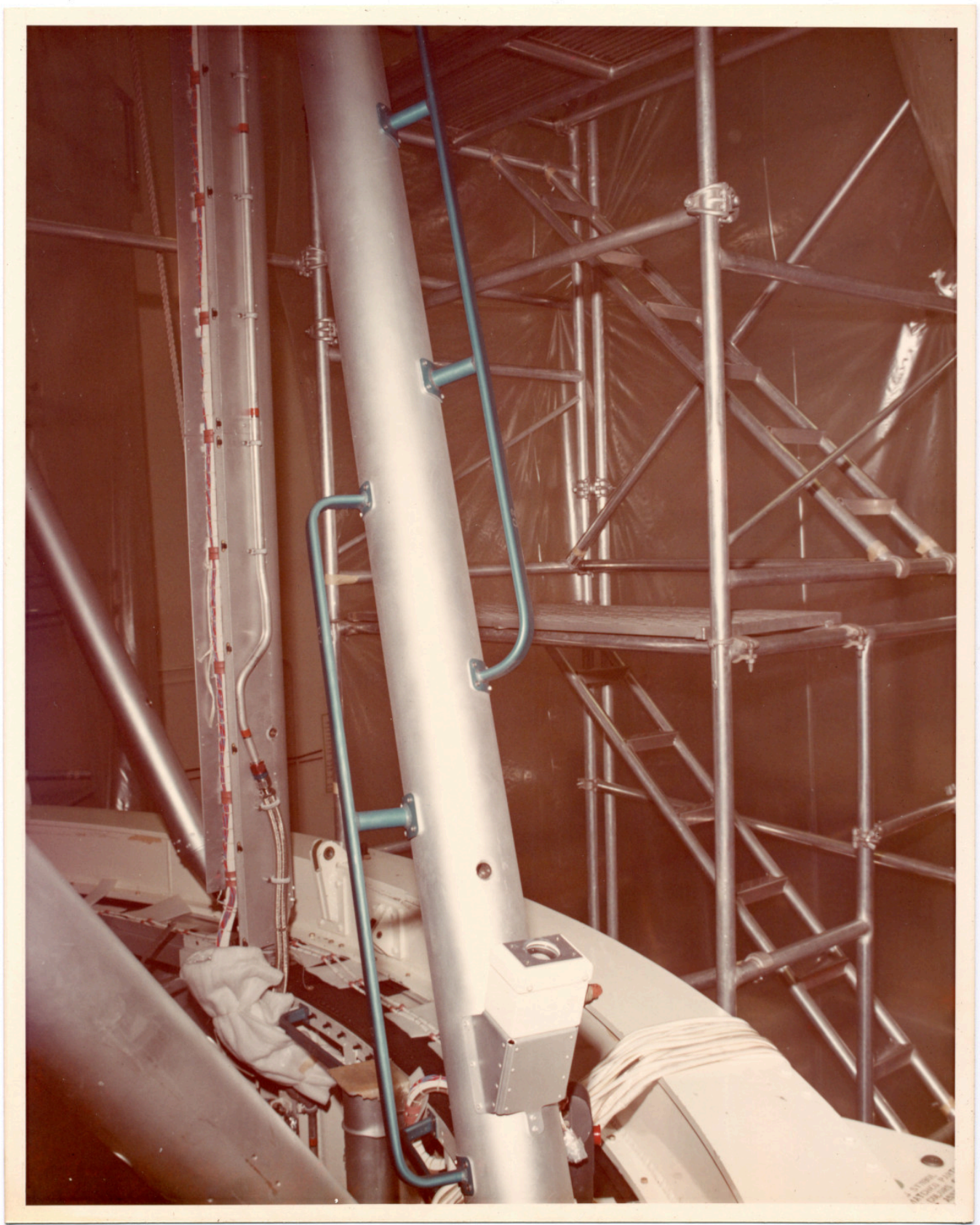
There is a still caption on the back which reads: "Airlock Zone 13 handrails D2 and D7 end EVA lift on lower DA -Y and +Z Quadrant, MDAC Input for month of June."
