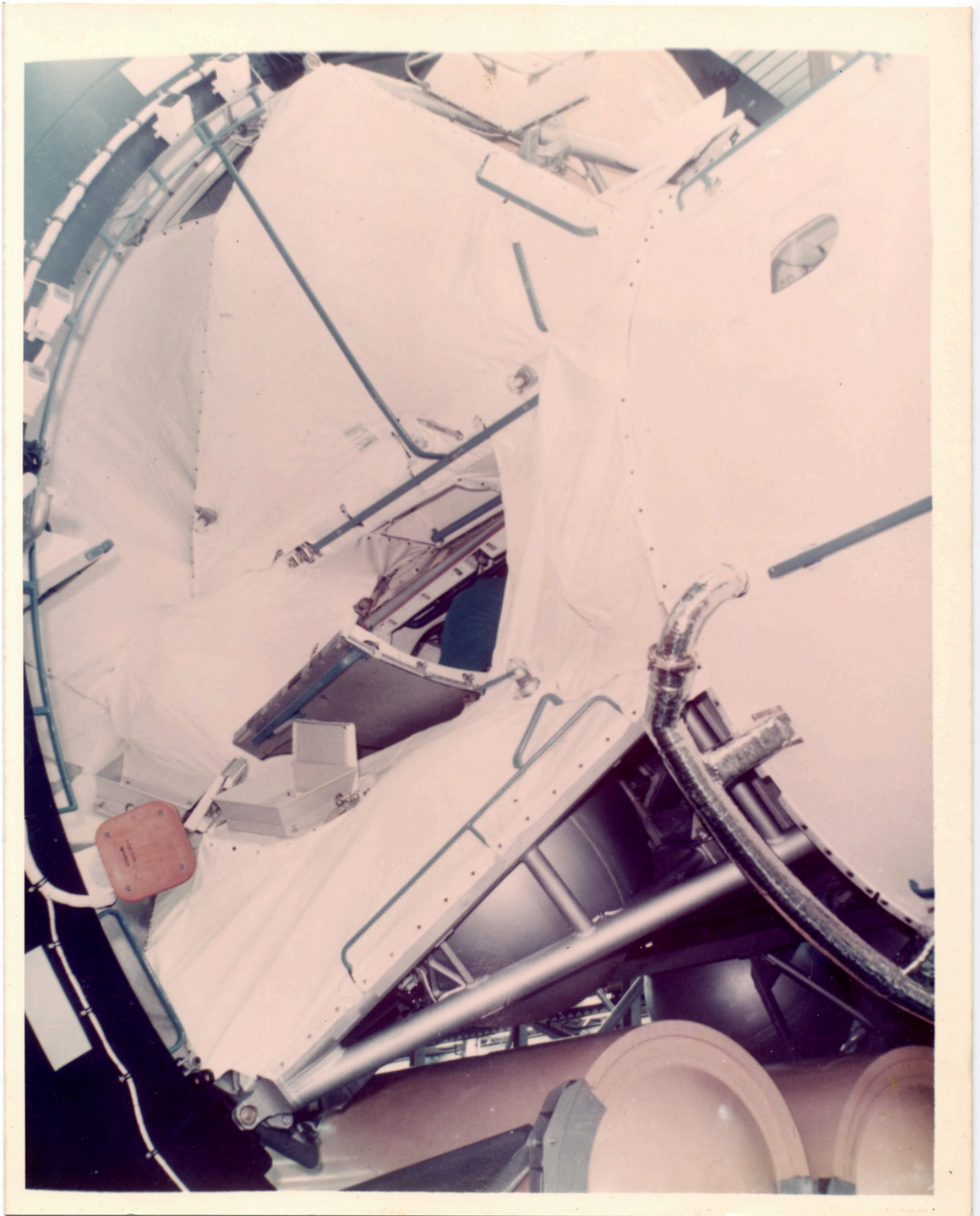
There is a still caption on the back which reads: "NEUTRAL BUOYANCY - SKYLAB-3 PRIME GREW EVA TRAINING - EV-2 PLACES S-082 PACKAGE IN RACK AT ATM SUN END."
