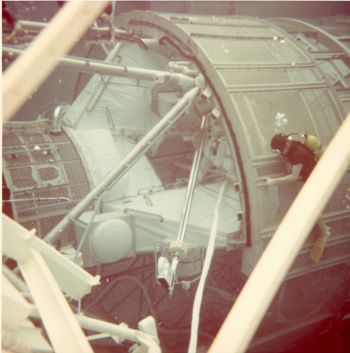
There is a still caption on the back which reads: "NEUTRAL BUOYANCY - ATM FILM RETRIEVAL - OVERALL VIEW OF EXTENDABLE BOOM EXTENDING FROM FAS TO ATM."
