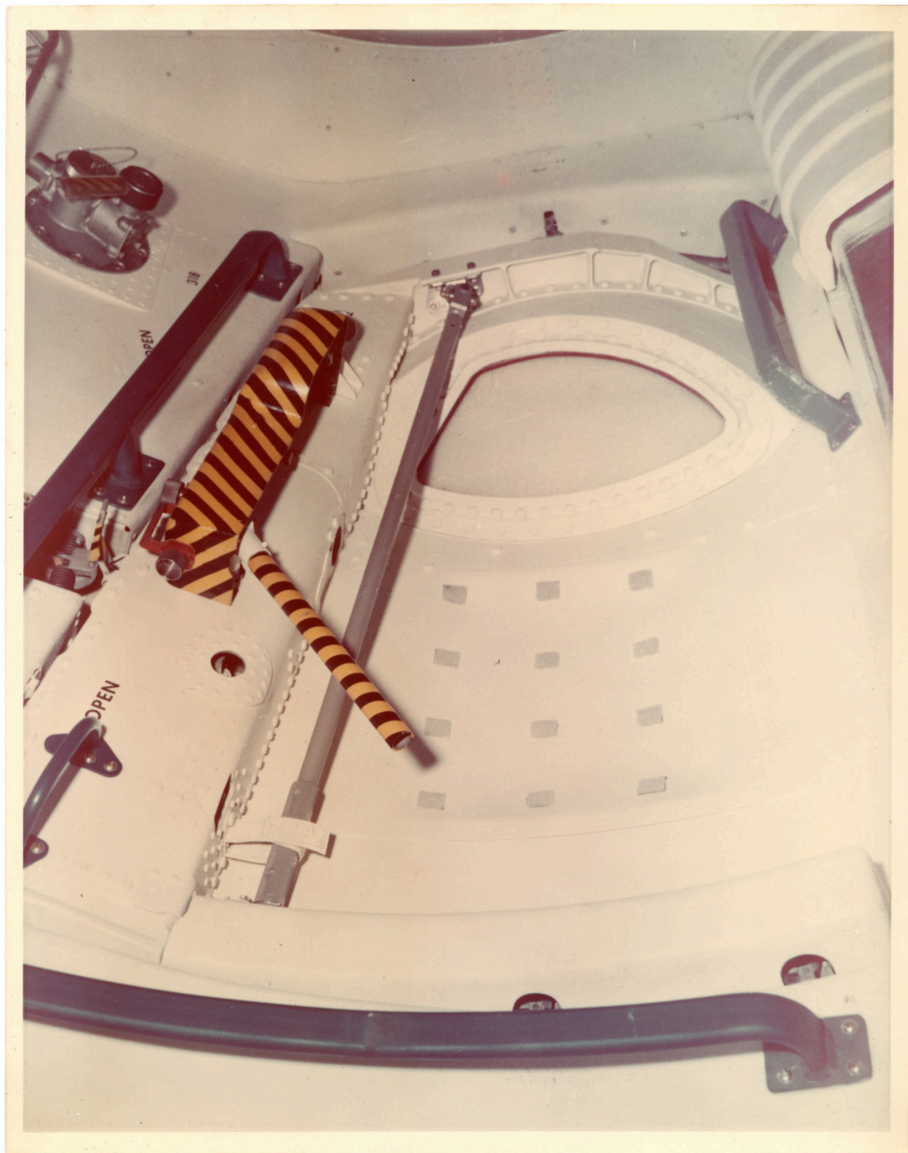
There is a still caption on the back which reads: "Airlock zone 14 & 6 temporary stowage hook. MDAC Input for month of June."
