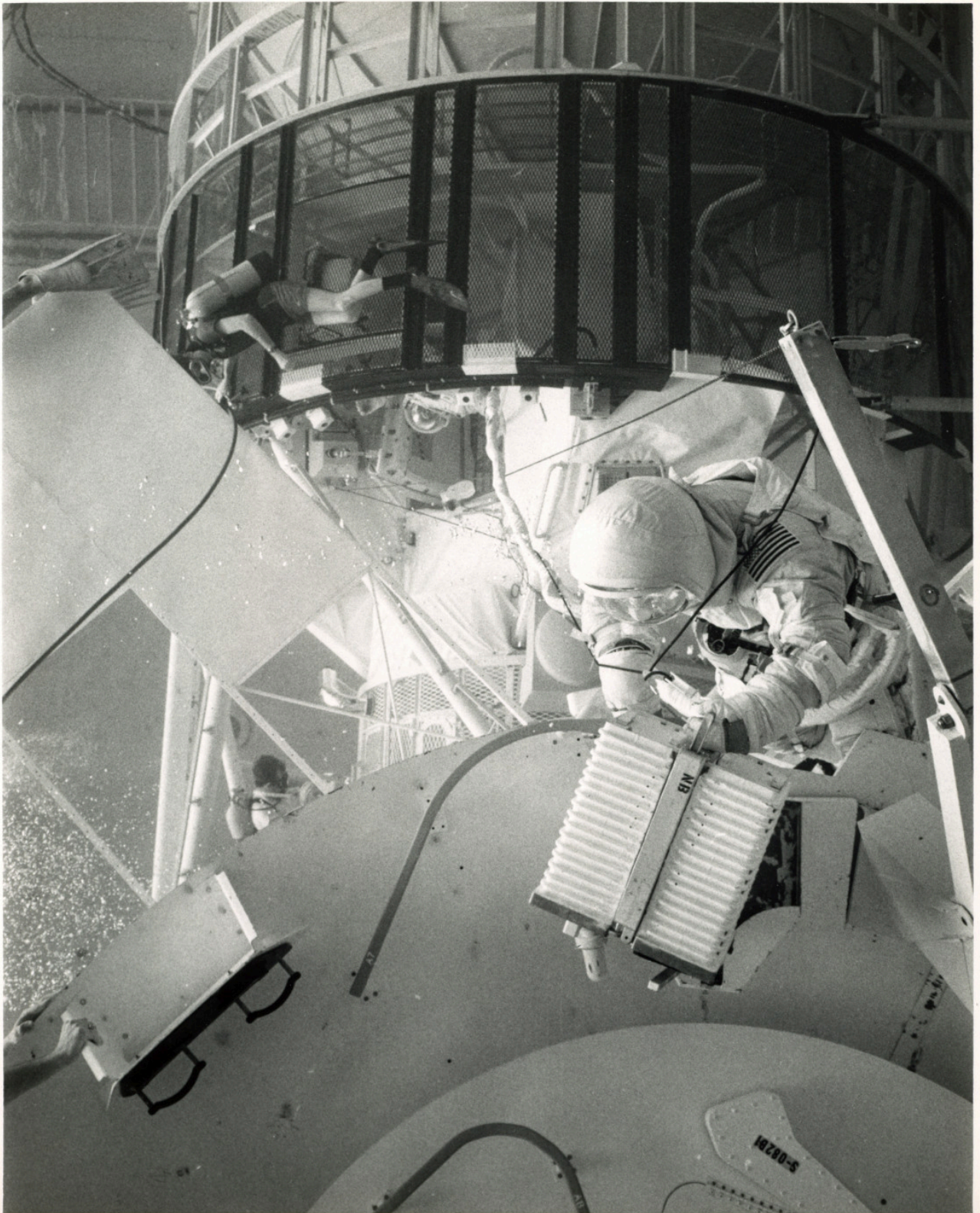
There is a still caption on the back which reads: "NEUTRAL BUOYANCY, SUBJECT ATTACHES CLOTHESLINE TO ATM SUN-END TRANSFER STATION."
