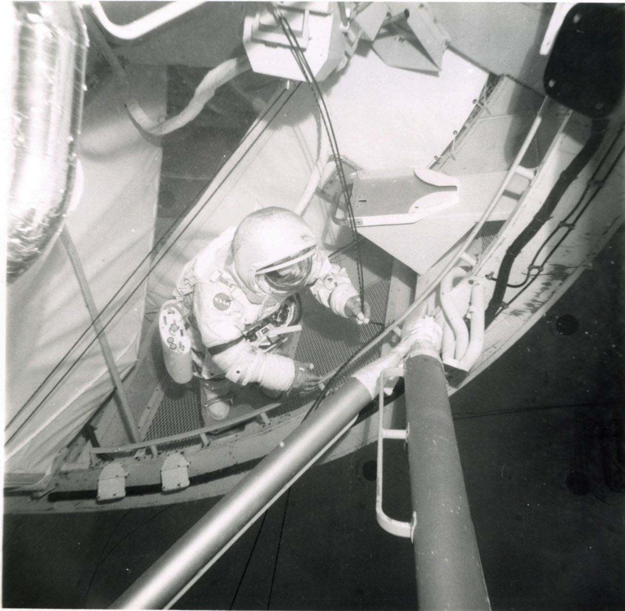
There is a still caption on the back which reads: "NEUTRAL BUOYANCY EVALUATION OF CLOTHESLINE CLIPS IN FAS AREA. VIEW -2."
