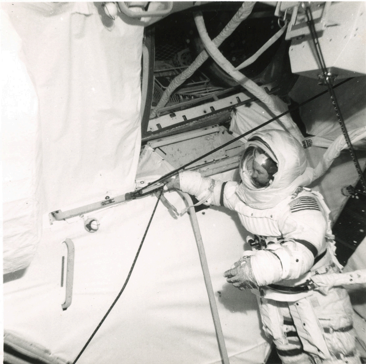
There is a still caption on the back which reads: "NEUTRAL BUOYANCY AIRLOCK HATCH AND CENTER WORKSTATION CLOTHESLINE INTERFERENCE VIEW -5."
