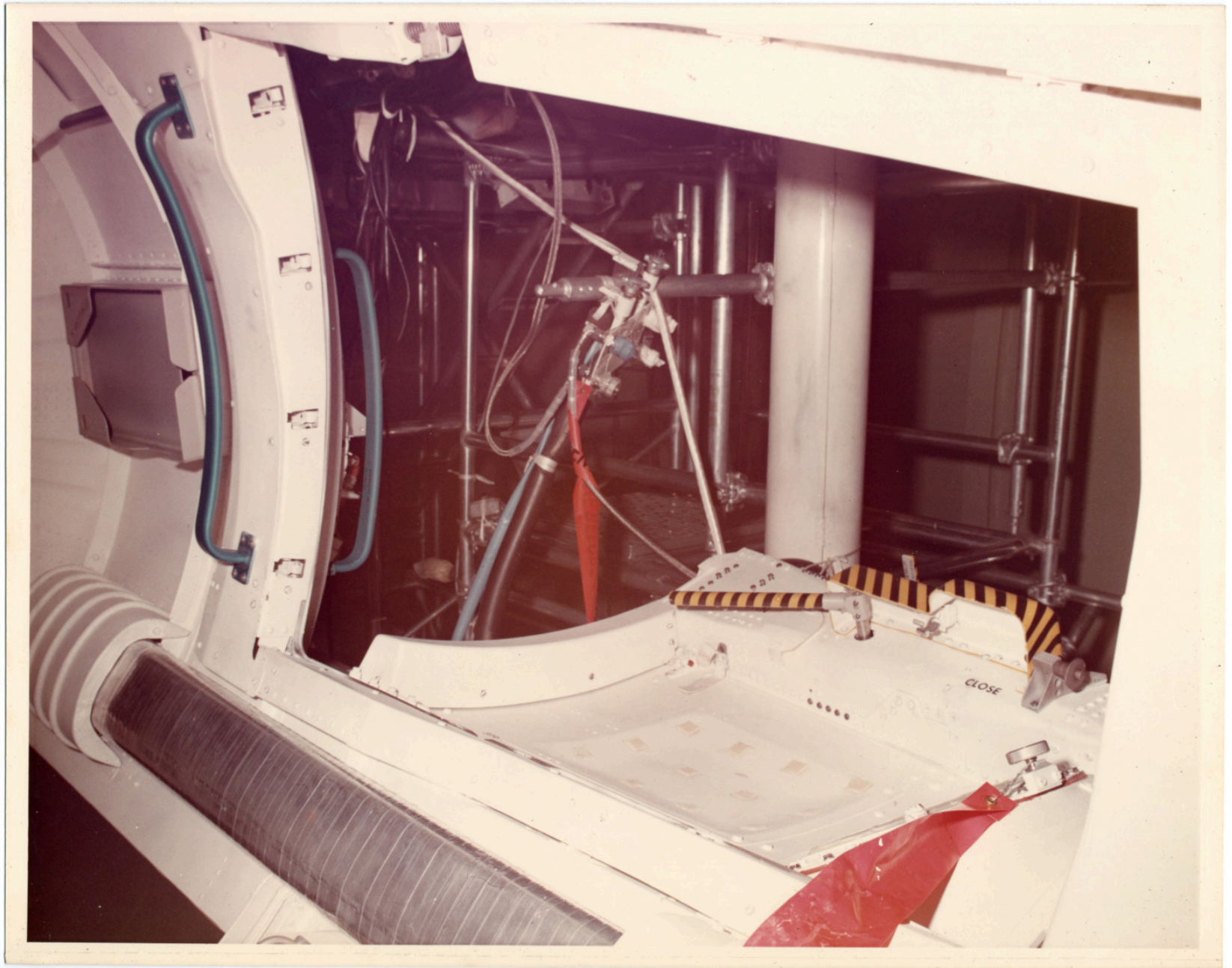
There is a still caption on the back which reads: "NASA TRAINER - OPEN EVA HATCH FROM EVA AREA. NASA-2595."
