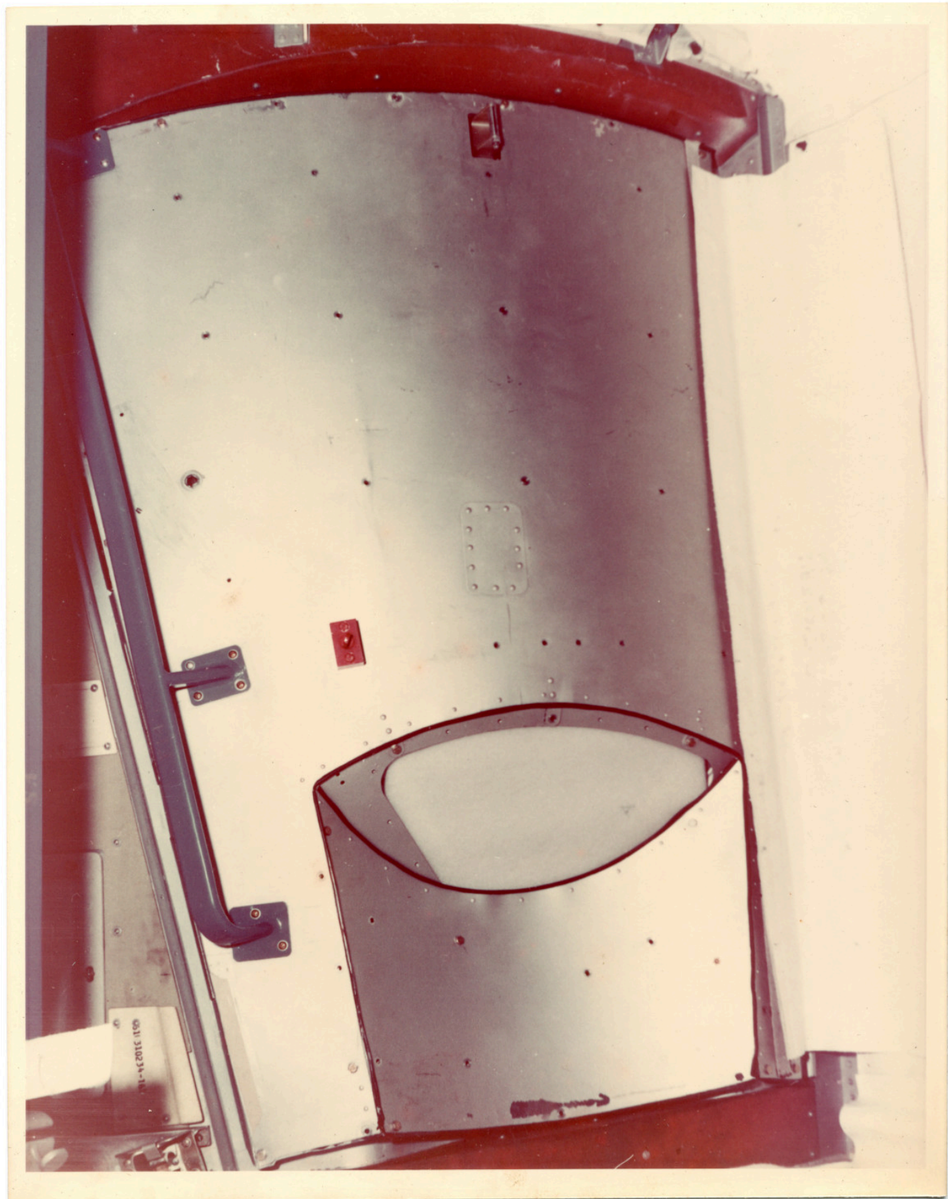
There is a still caption on the back which reads: "Airlock Zone 6 between zones 8&9 closeup of EVA hatch from outside vehicel with hatch open. MDAC Input for month of June."
