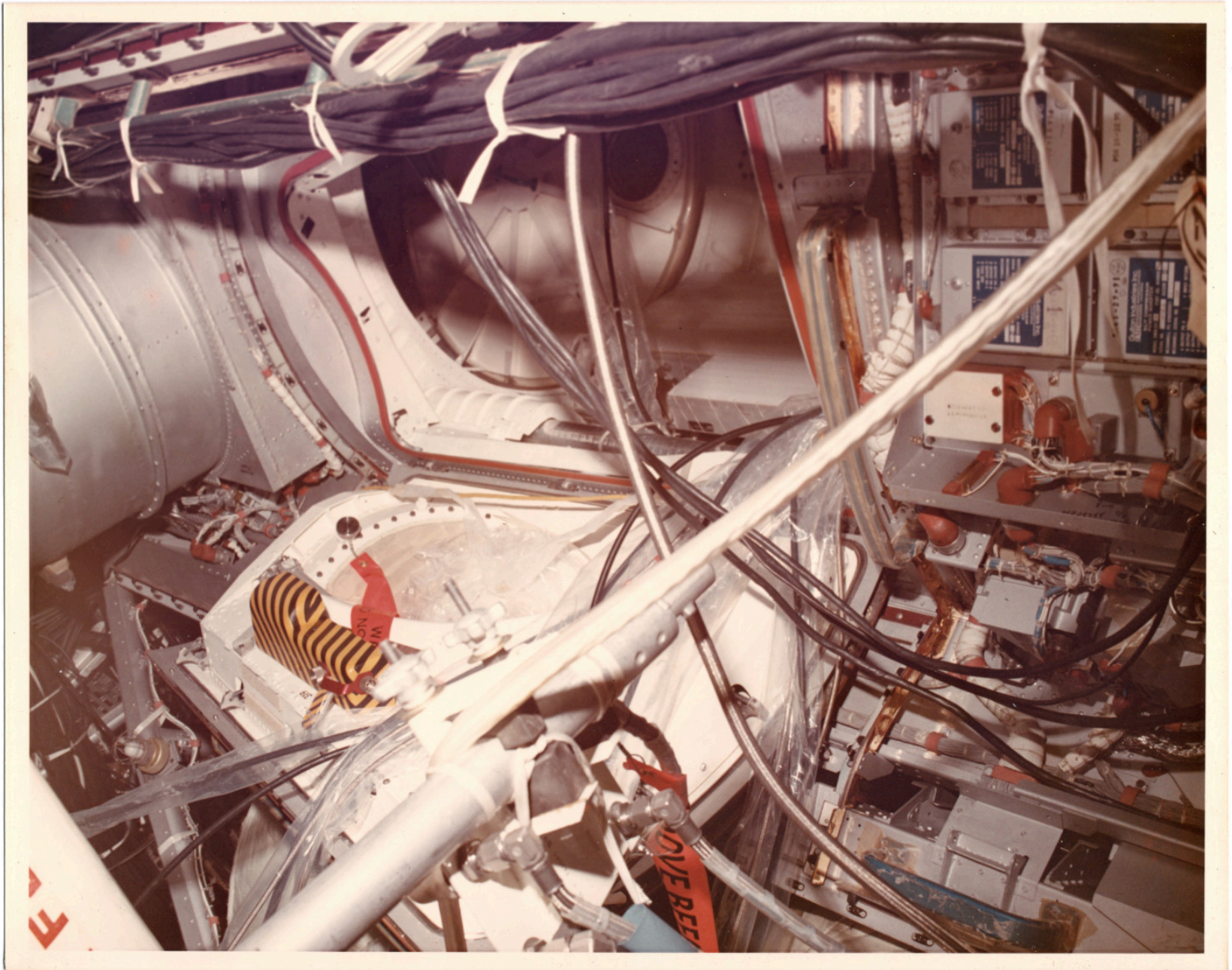
There is a still caption on the back which reads: "AIRLOCK - ZONE - 3. CLOSEUP OF EVA HATCH OPEN - VIEW ANGLED FROM FORWARD SECTION OF LOCK COMPARTMENT LOOKING AFT. MDAC INPUT FOR JUNE."
