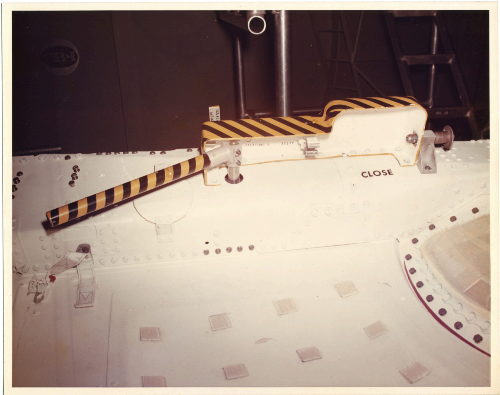
There is a still caption on the back which reads: "AIRLOCK-ZONE-3. CLOSEUP OF EVA HATCH OPEN-VIEW STRAIGHT OUT FROM INSIDE LOCK COMPARTMENT, MDAC INPUT FOR JUNE."
