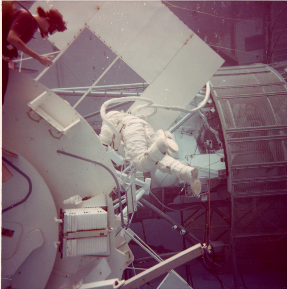
There is a still caption on the back which reads: "NEUTRAL BUOYANCY OVERALL VIEW OF SUN-END CLOTHESLINE DEPLOYED SHOWING SAG IN LINE, VIEW -1."
