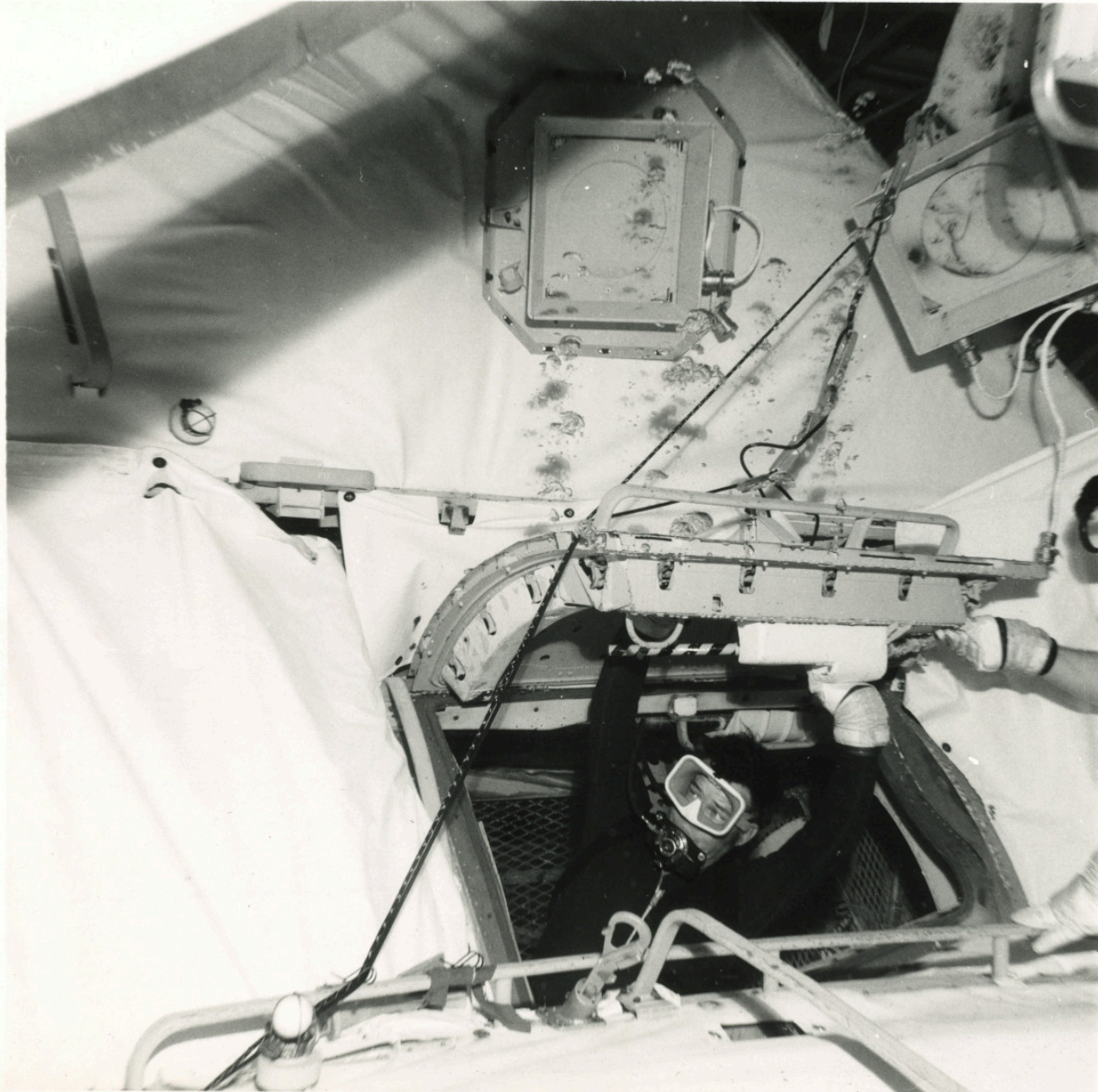
There is a still caption on the back which reads: "NEUTRAL BUOYANCY - SKYLAB -3 BACKUP CREW EVA TRAINING - 3-082 PACKAGE RETRIEVAL SHOWING 16MM DAC CAMERA KNOCKED OUT OF POSITION BY RV-1'S HEAD AND SHOULDER"
