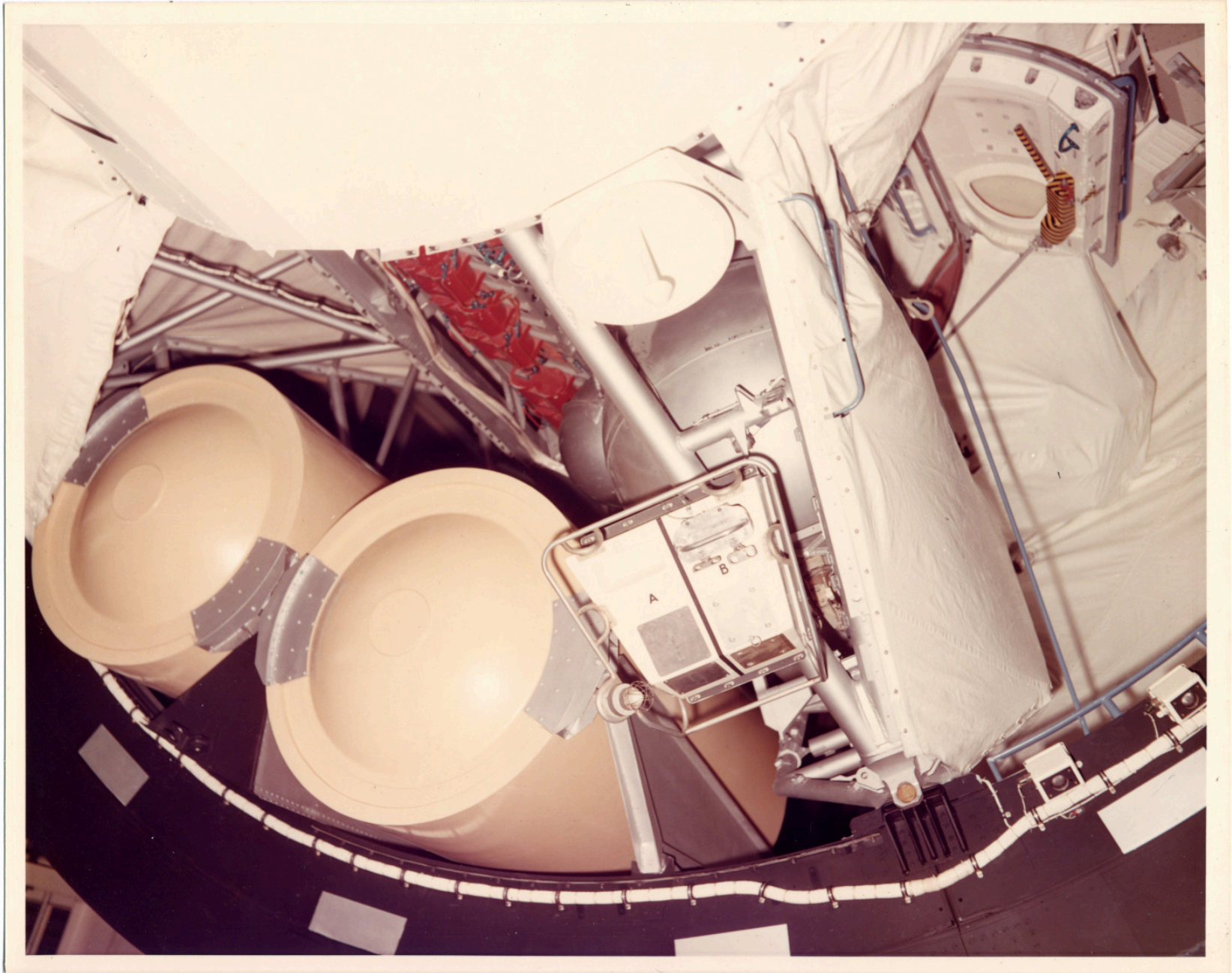
There is a still caption on the back which reads: "AIRLOCK NASA TRAINER ON PRODUCTION LINE IN MDAC-E BLDG-101 EXTERIOR VIEW SHOWING D024 EXPERIMENT MODULE, O2 TANKS & EVA AREA. NASA-1434"
