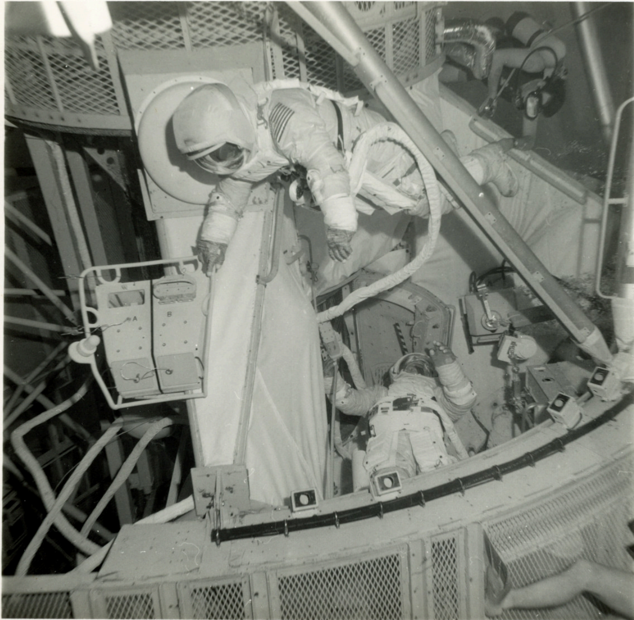
There is a still caption on the back which reads: "NEUTRAL BOUYANCY, ASTRONAUT GIBSON, ED APPROACHING EXPERIMENT DO-24 DURING SETURN TRANSIATION FROM ATM, MUSGRAVE AT AIRLOCK WORKSTATION."
