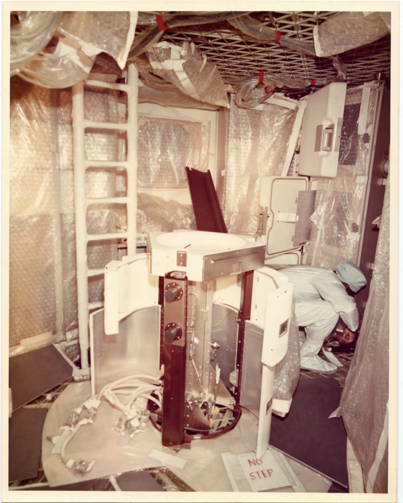
There is a still caption on the back which reads: "VIEW OF WARDROOM AREA IN OWS NO 1"
