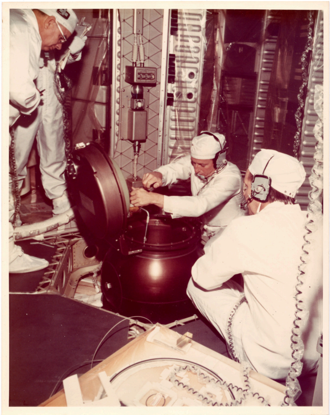
There is a still caption on the back which reads: "ASTRONAUT CONRAD SECURING INNER CYLINDER OF TRASH DISPOSAL AIRLOCK. OWS NO-1."
