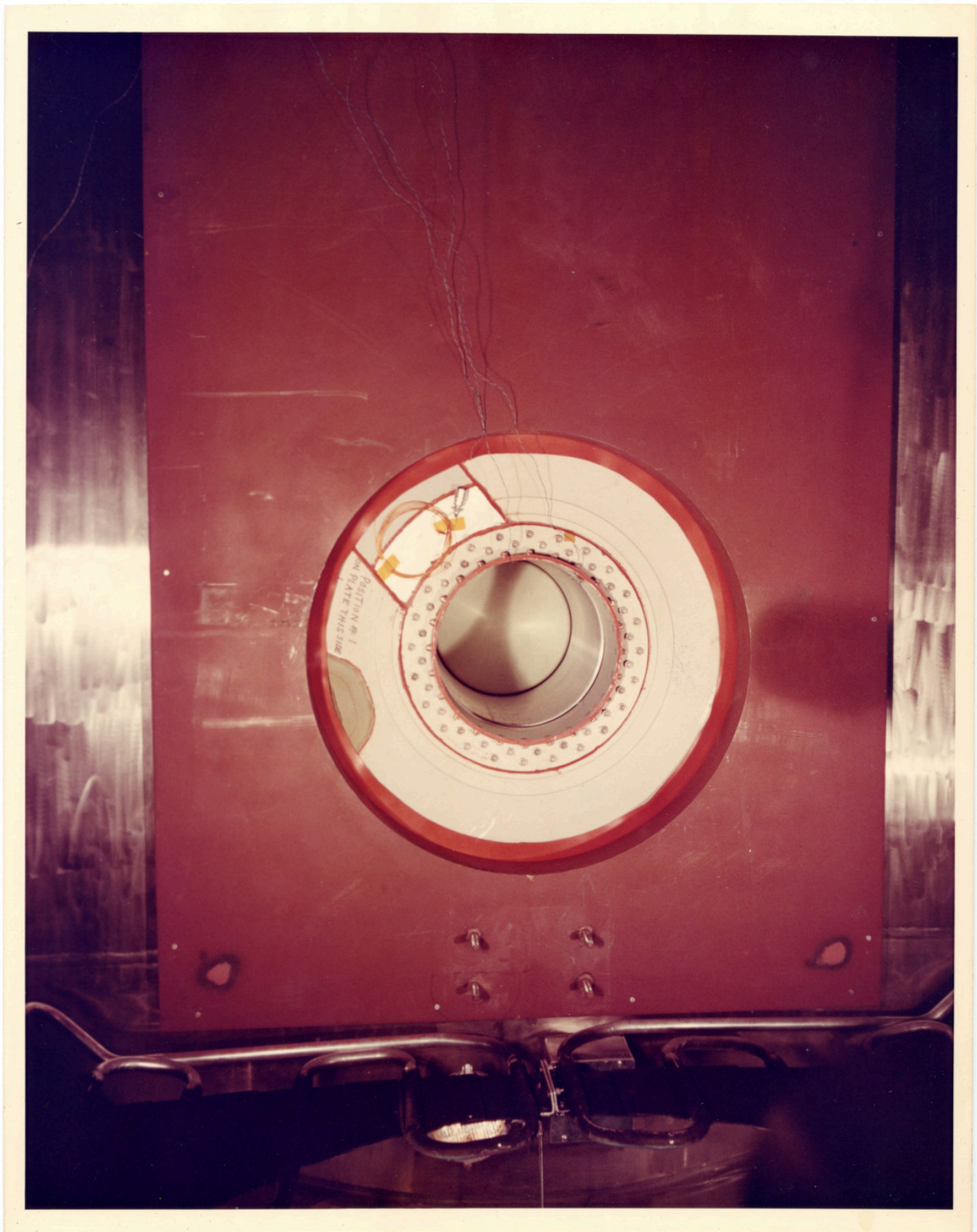
There is a still caption on the back which reads: "TRASH DISPOSAL AIRLOCK AFTER EJECTION CYCLE WITH EJECTION DEVICE RETRACTED. OWS"
