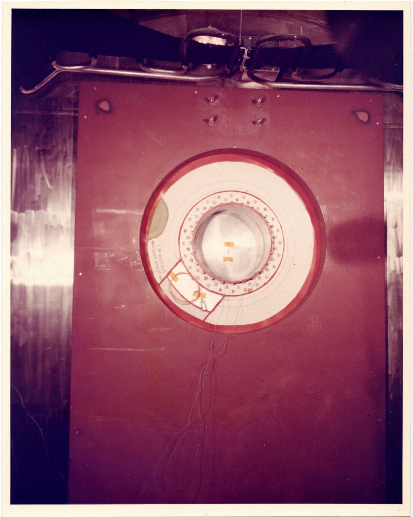
There is a still caption on the back which reads: "OUTBOARD SIDE OF AIRLOCK TEST SPECIMEN DURING TESTING WITH OUTBOARD VALVE IN CLOSED POSITION OWS."
