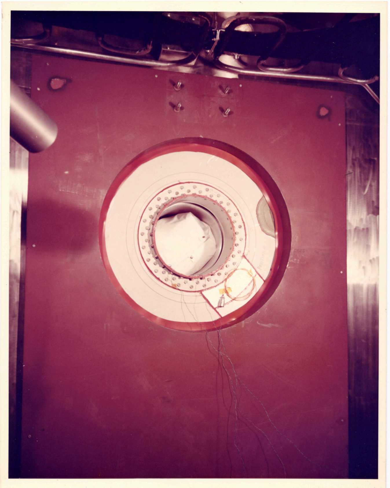
There is a still caption on the back which reads: "OUTBOARD SIDE OF AIRLOCK TEST SPECIMEN DURING TESTING WITH OUTBOARD VALVE IN OPEN POSITION OWS."
