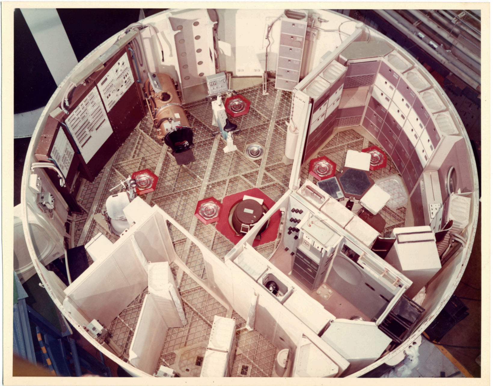
There is a still caption on the back which reads: "SKYLAB I-G TRAINER CREW QTRS, CLOCKWISE EXPERIMENT WORK AREA, WARD ROOM WASTE MANAGEMENT, SLEEP COMPARTMENT."
