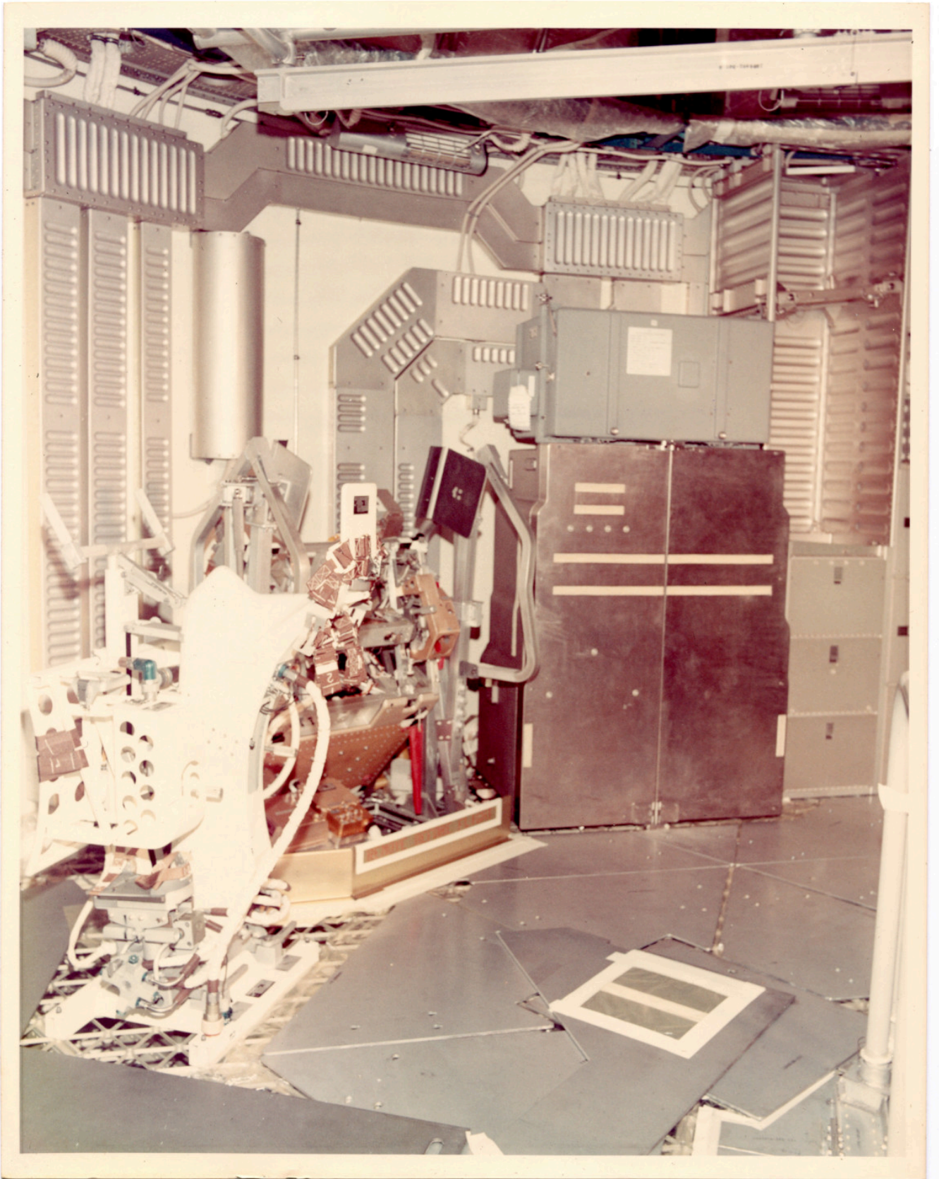
There is a still caption on the back which reads: "M509 AND T020 EXPERIMENTS. FILM VAULT, AND S-63 EXPERIMENT CONTAINER ON TOP OF FILM VAULT. OWS NO. 1."
