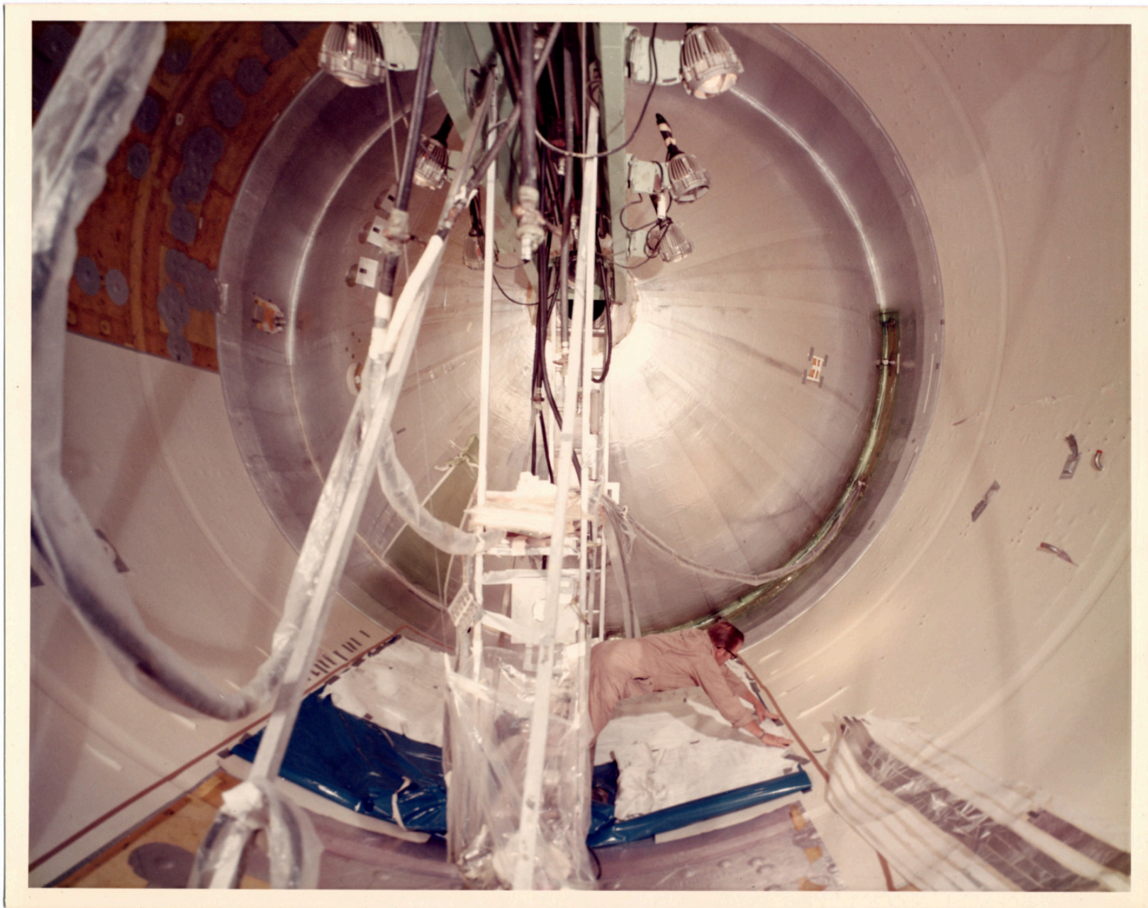
There is a still caption on the back which reads: "INTERIOR VIEW OF OWS BACKUP LOOKING AFT, AS ASSEMBLER PLACES BLUE [illegible] MATERIAL OVER LINER SECTION PRIOR TO 24-HOUR VACUUM CURB."
