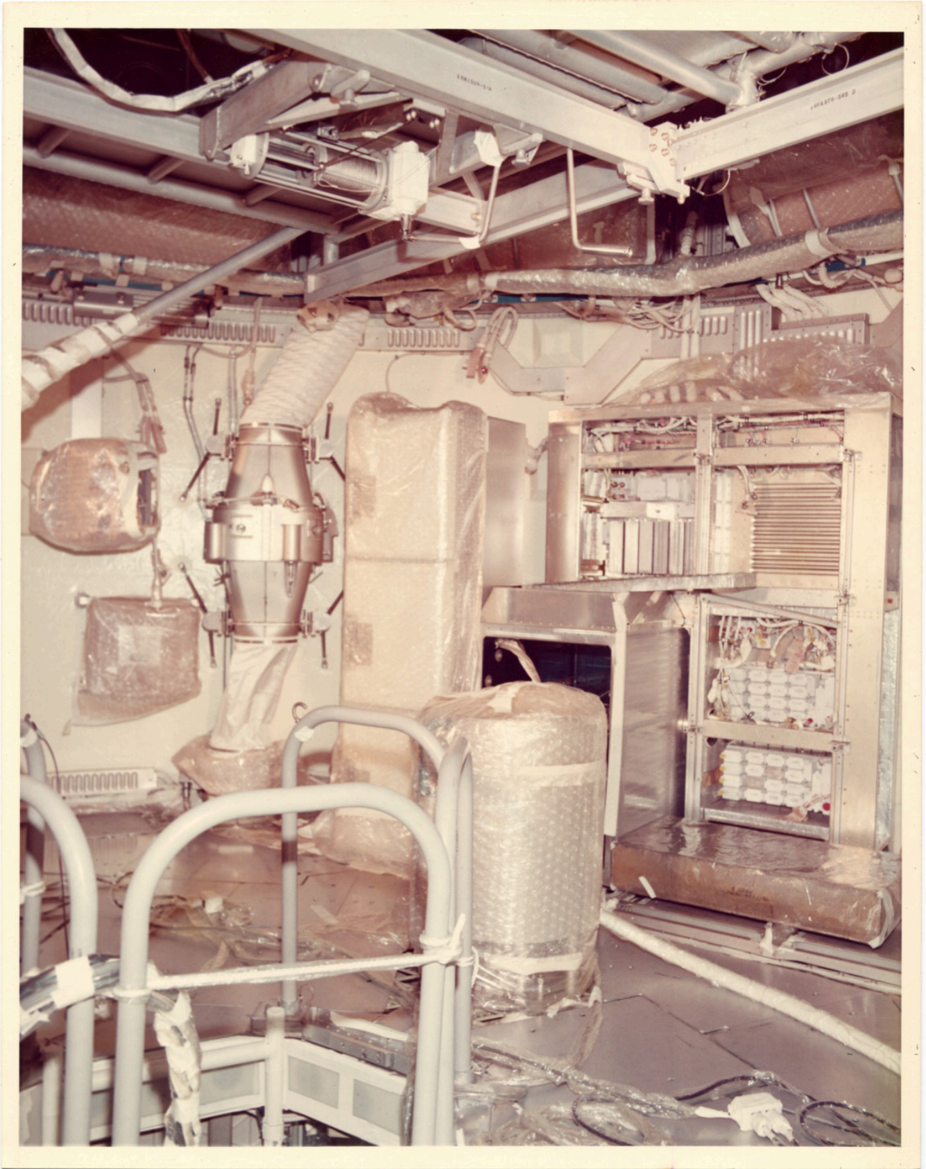
There is a still caption on the back which reads: "FAN CLUSTER. FOOD FREEZER REFIGETATION SUBSYSTEM IN UPPER LEVEL. OWS NO. 1"
