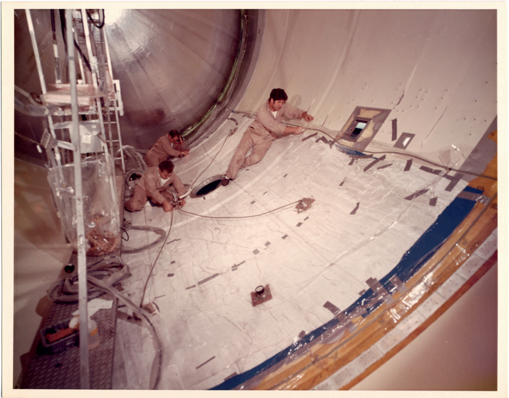
There is a still caption on the back which reads: "OVERALL VIEW OF INSIDE OF OWS BACKUP HABITATION CYLINDER AS X ASSEMBLERS VACUUM BAG SECTION OF ALUMINUM FOIL/TEFLON LINER. (LOOKING AFT)"
