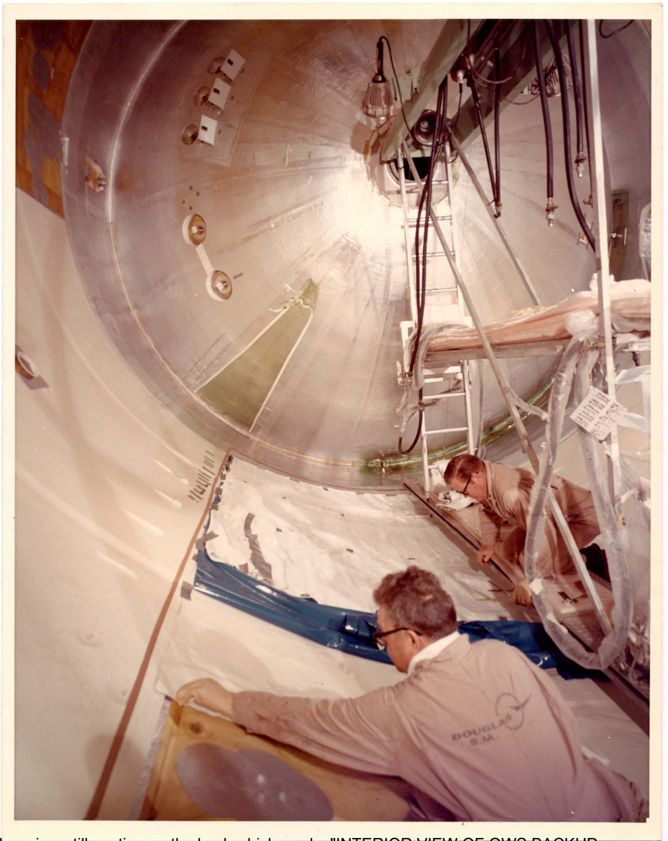
There is a still caption on the back which reads: "INTERIOR VIEW OF OWS BACKUP HABITATION CYLINDER AS TECNITIONS VACUUM BAG ANOTHER SECTION OF ALUMINUM FOIL/TEFLON LINER TO WALL INSULATION OF SPACECRAFT."
