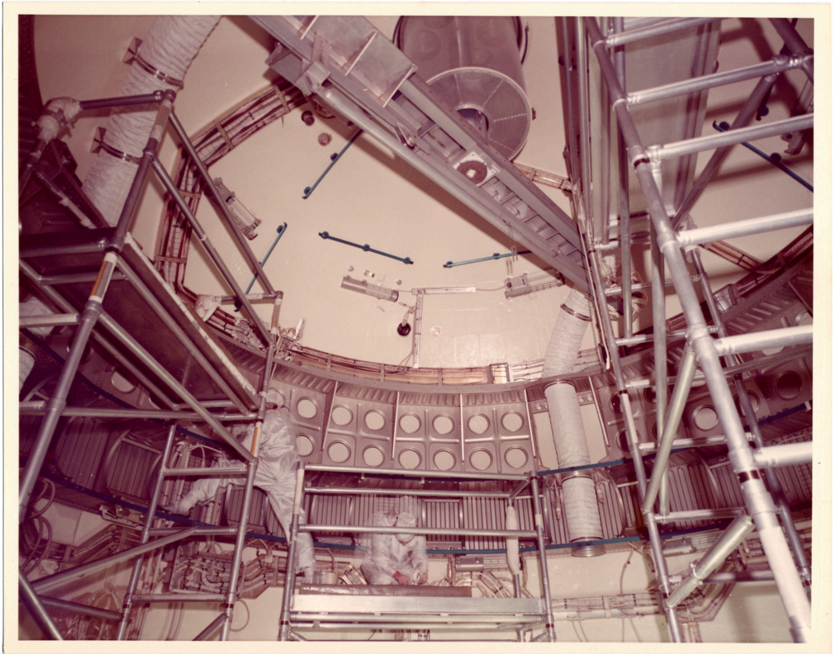
There is a still caption on the back which reads: "UPPER STORAGE & EXPERIMENTAL AREA. INSTALLATION OF WIRE HARNESS BELOW WATER CONTAINER SUPPORT STRUCTURE."
