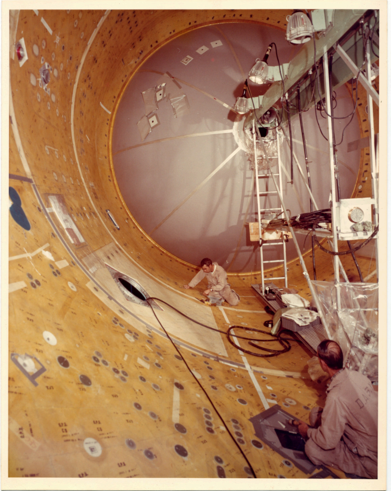
There is a still caption on the back which reads: "BONDING SUPPORT DISCS TO WALL OF SPACECRAFT OWS BACKUP"
