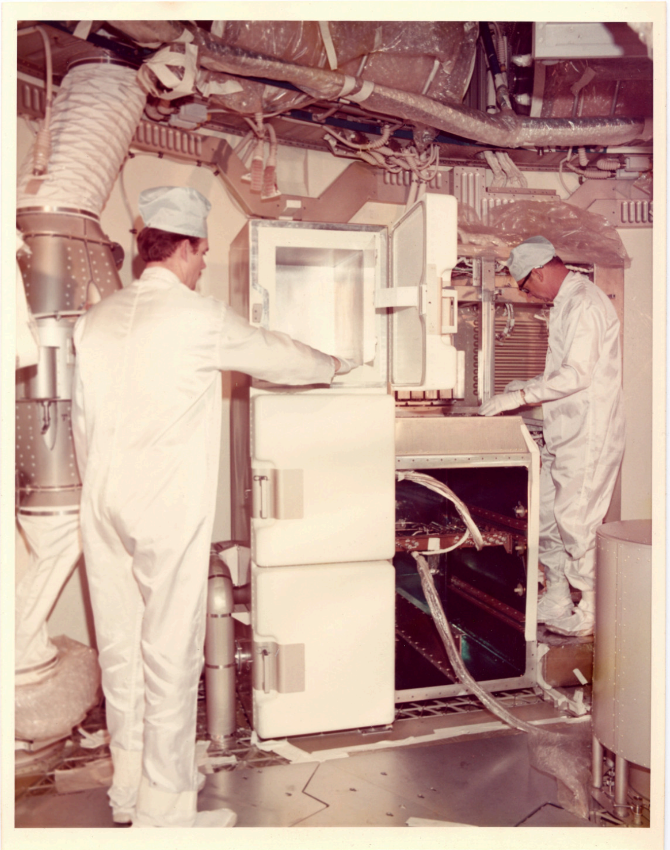
There is a still caption on the back which reads: "INSPECTING FOOD FREEZER & REFRIGERATION SUBSYSTEM IN UPPER LEVEL OF OWS NO. 1."
