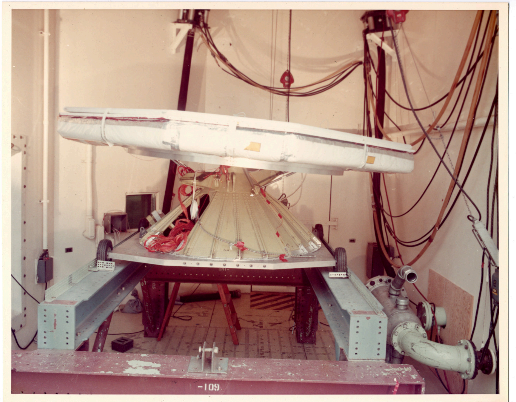
There is a still caption on the back which reads: "ACCOUSTIC TESTING SET-UP WITH OWS RADIATOR AND PLUME SHIELD INSTALLED ON FIXTURE."
