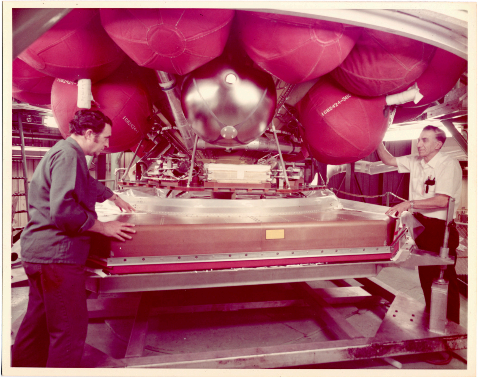
There is a still caption on the back which reads: "PRE-FIT OF RADIATOR FOR REFRIGERATION SUBSYSTEM BEING CONDUCTED OWS-NO-1."
