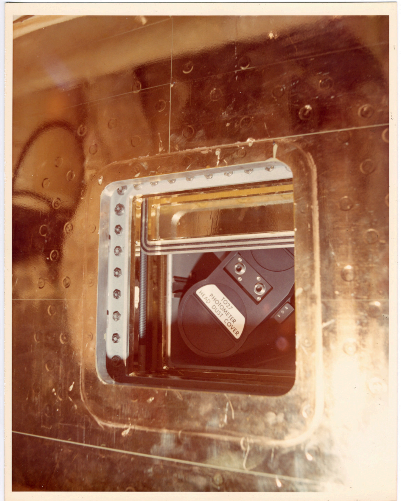
There is a still caption on the back which reads: "COVERED TO-27 PHOTOMETER AS SEEN THROUGH SCIENTIFIC AIRLOCK FROM OUTSIDE OWS NO-1."
