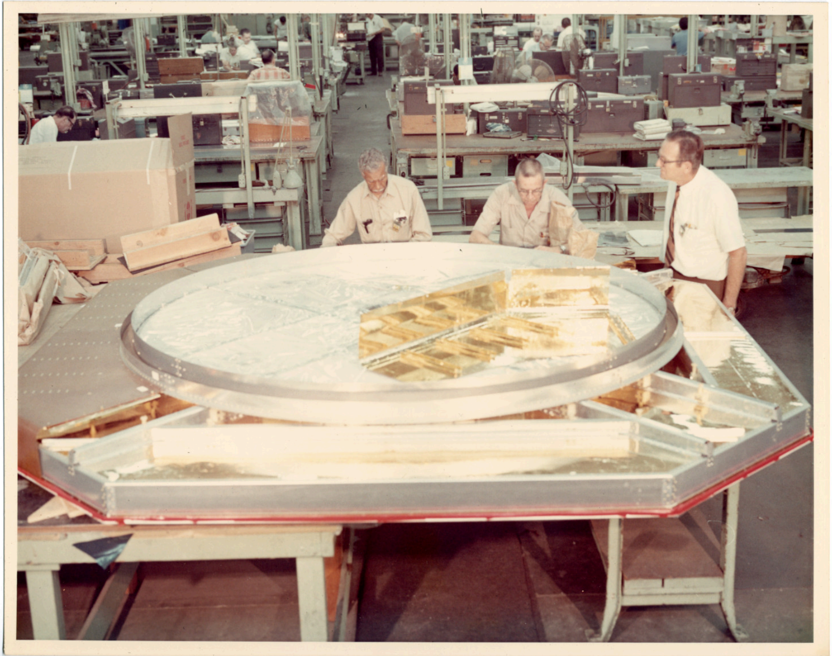
There is a still caption on the back which reads: "INSTALLING PRESSURE-SENSITIVE GOLD TAPE ON OWS RADIATOR STRUCTURE DURING FABRICATION AT SANTA MONICA FACILITY. OWS AUG. 1971 INPUT."
