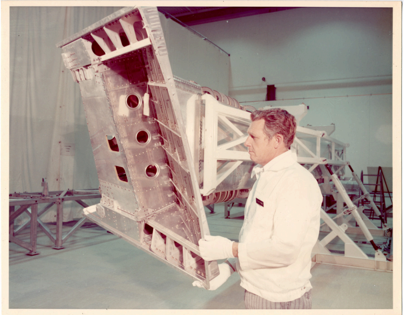
There is a still caption on the back which reads: "FORWARD FAIRING FITTING FOR SAS IN FULL DEPLOYED POSITION. OWS NO. 1. MDAC-INPUT"
