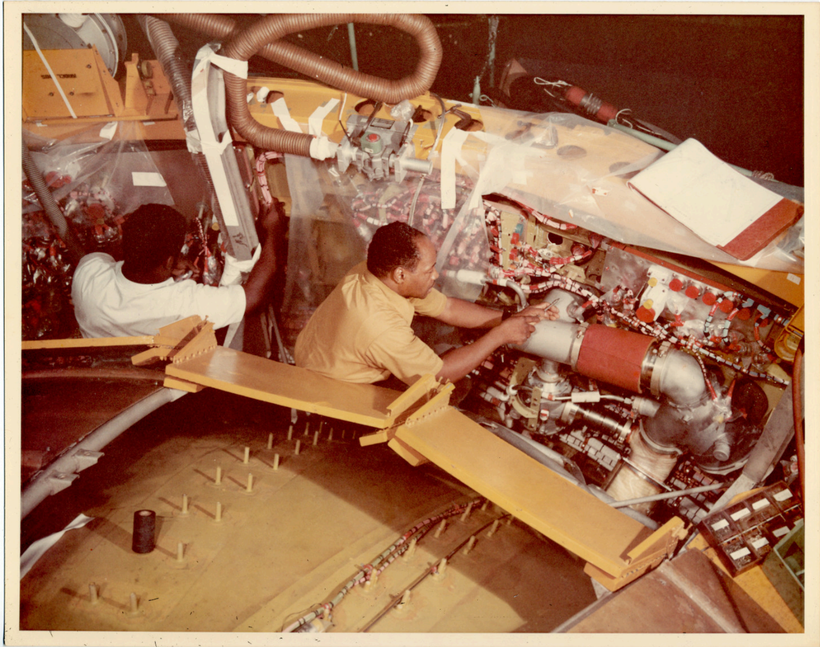
There is a still caption on the back which reads: "INSTALLING ELECTRICAL HARNESSSES ON FORWARD SKIRT OF OWS #1. AUG. 1971 INPUT."
