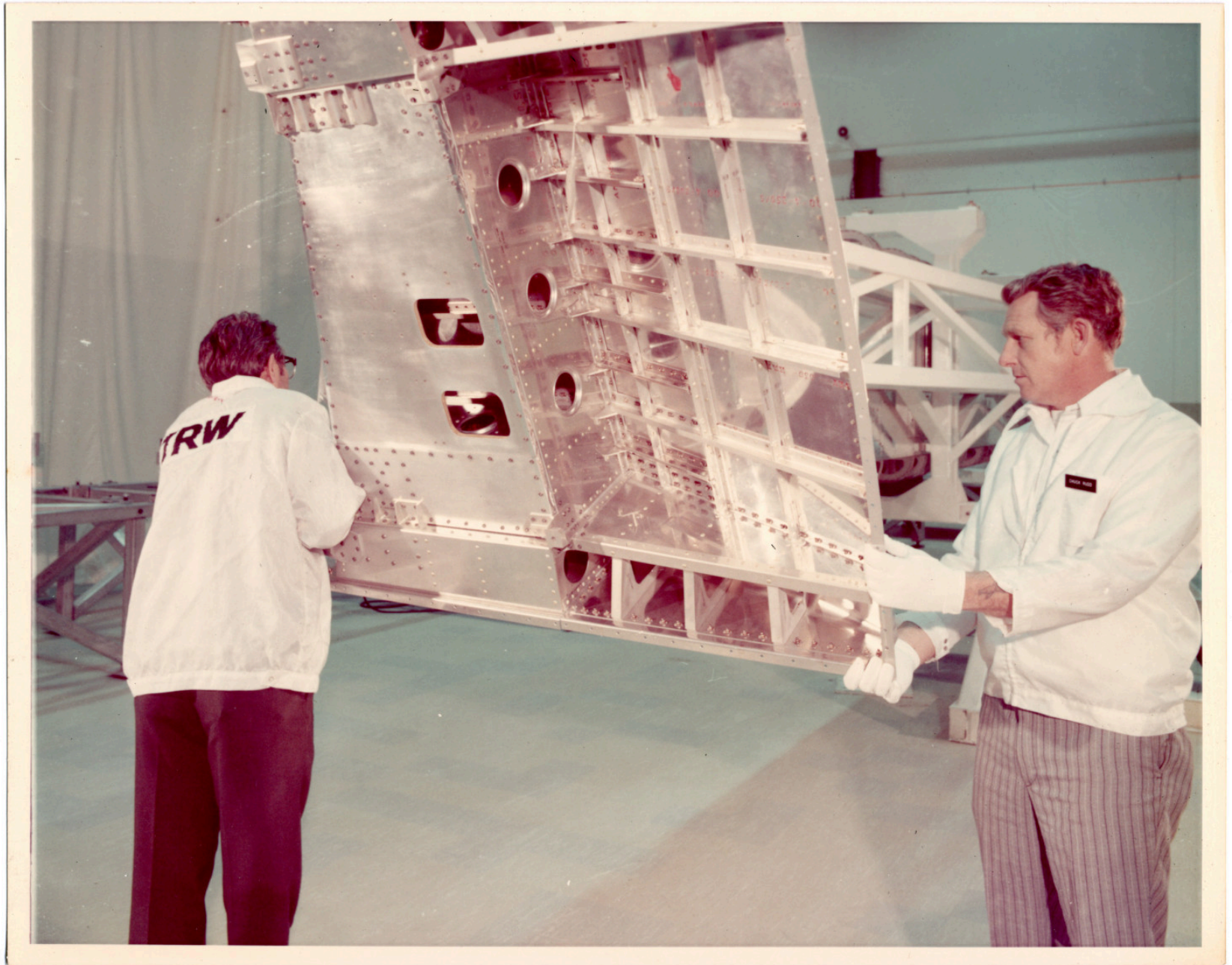
There is a still caption on the back which reads: "FORWARD FAIRING FOR SAS IN THREE-QUARTER DEPLOYED POSITION. OWS NO. 1. MDAC-INPUT"
