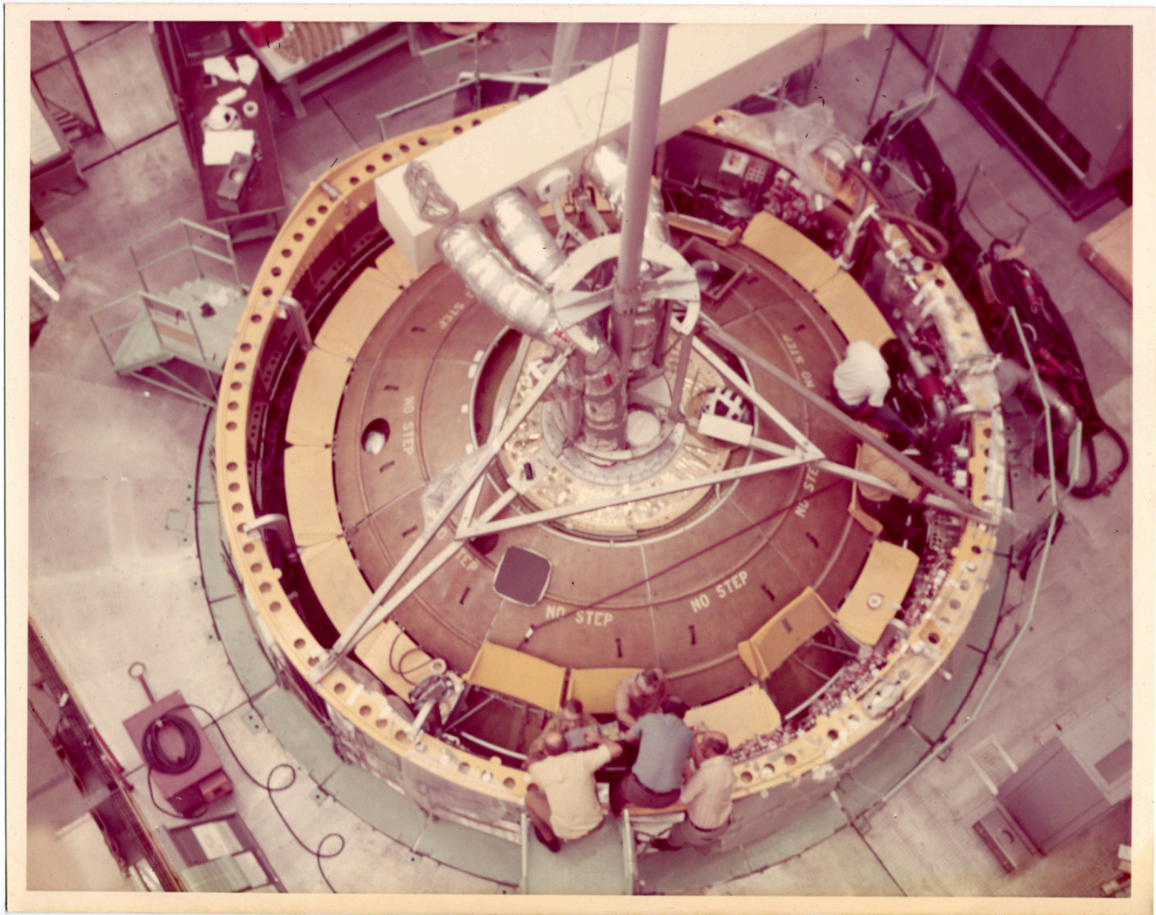
There is a still caption on the back which reads: "FORWARD SKIRT AND DOME AREA OF OWS #1 SPACECRAFT DURING INSTALLATION OF WIRE HARNESS AUG. 1971 INPUT."
