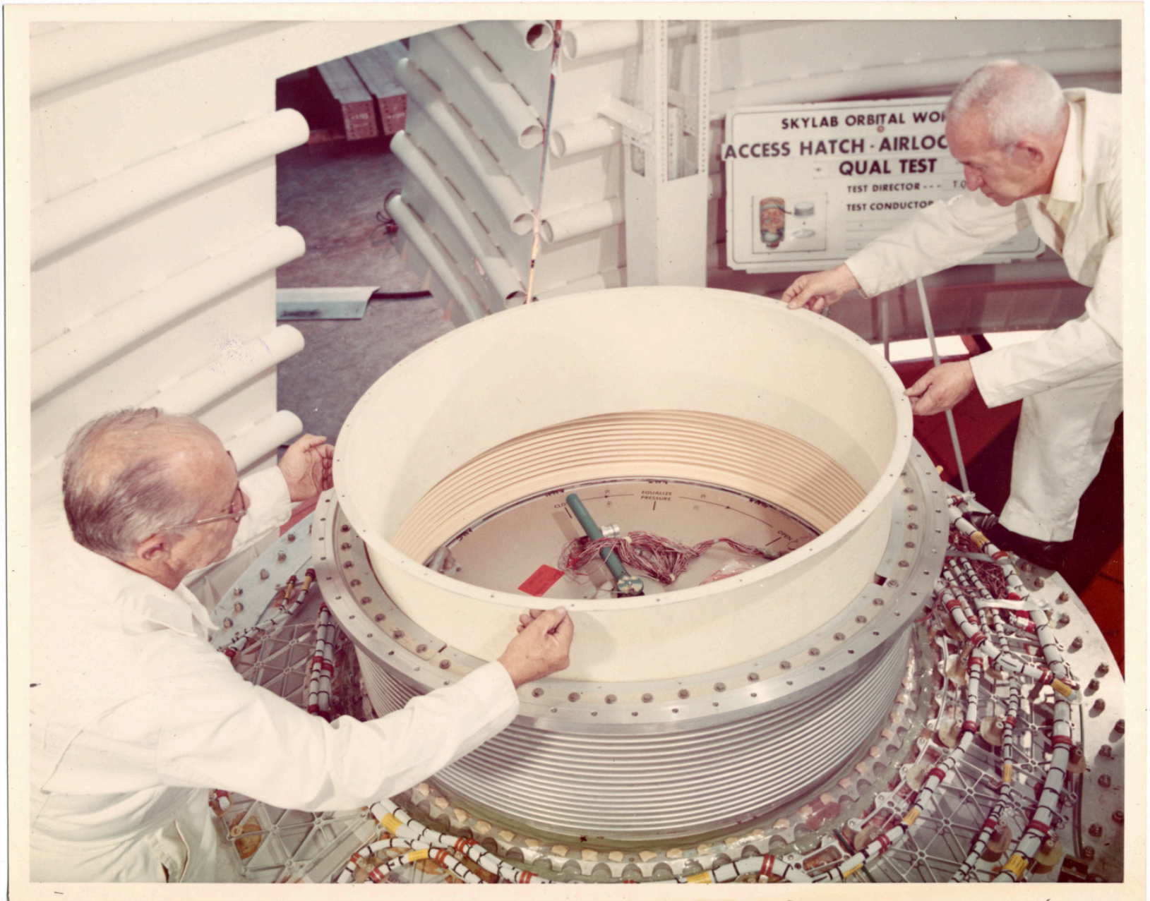
There is a still caption on the back which reads: "INSTALLING BELLOWS SLEEVE IN BELLOWS ASSEMBLY. OWS INPUT FOR SEPT 1971."
