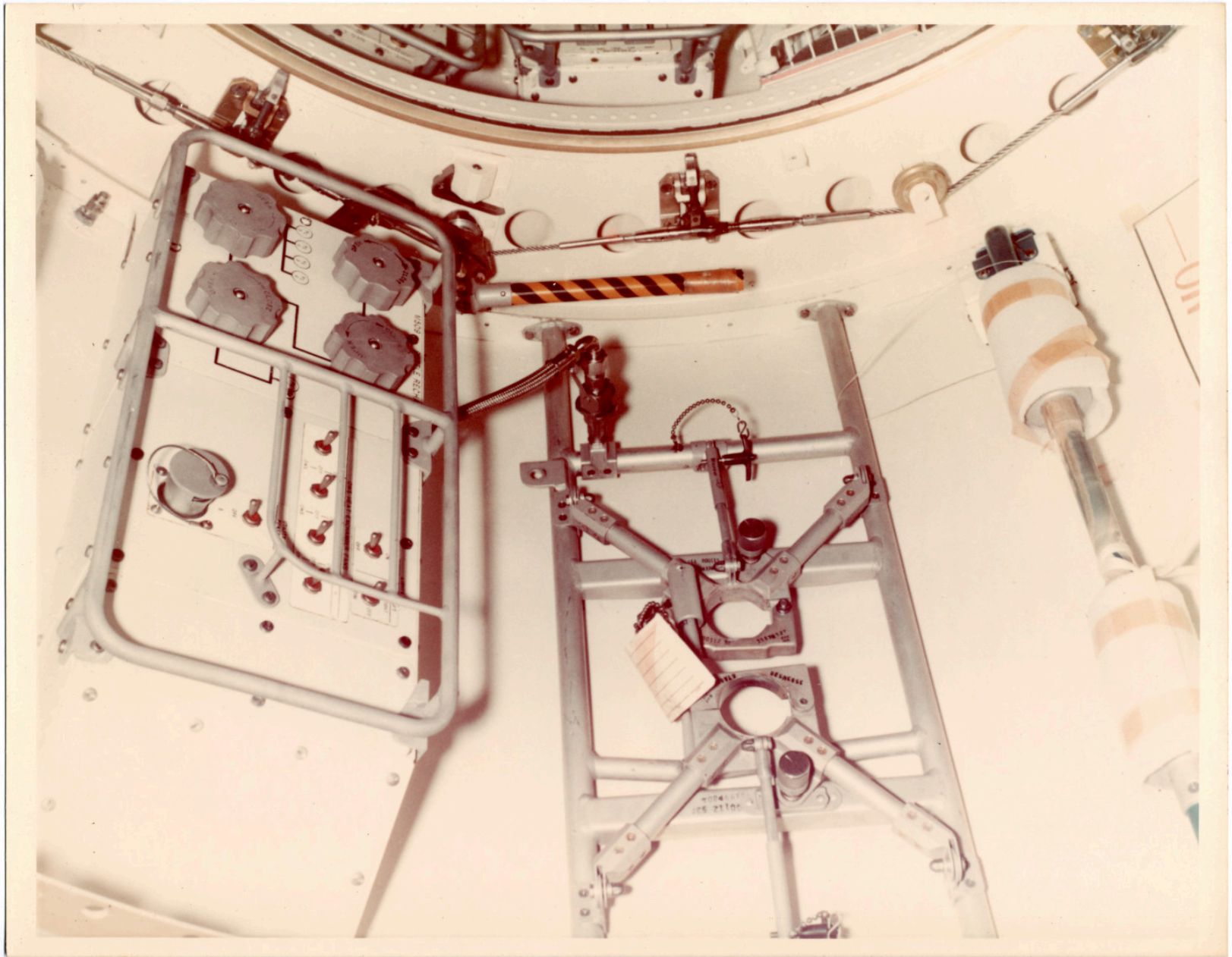
There is a still caption on the back which reads: "EXPERIMENT M509 NITROGEN RECHARGE STATION IN AFT COMPARTMENT OF U-1 AIRLOCK."
