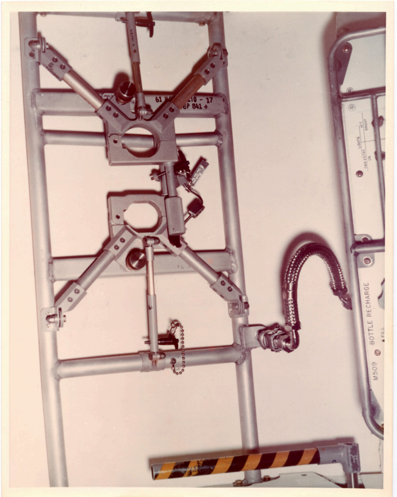
There is a still caption on the back which reads: "AIRLOCK NASA TRAINER ON PRODUCTION LINE IN MDAC-EAST BLDG. -101 FIT CHECK OF EXPERIMENT M509 RECHARGE STATION BRACKET IN STOWED CONFIGURATION. AUG. 1971 INPUT. NASA-1333."
