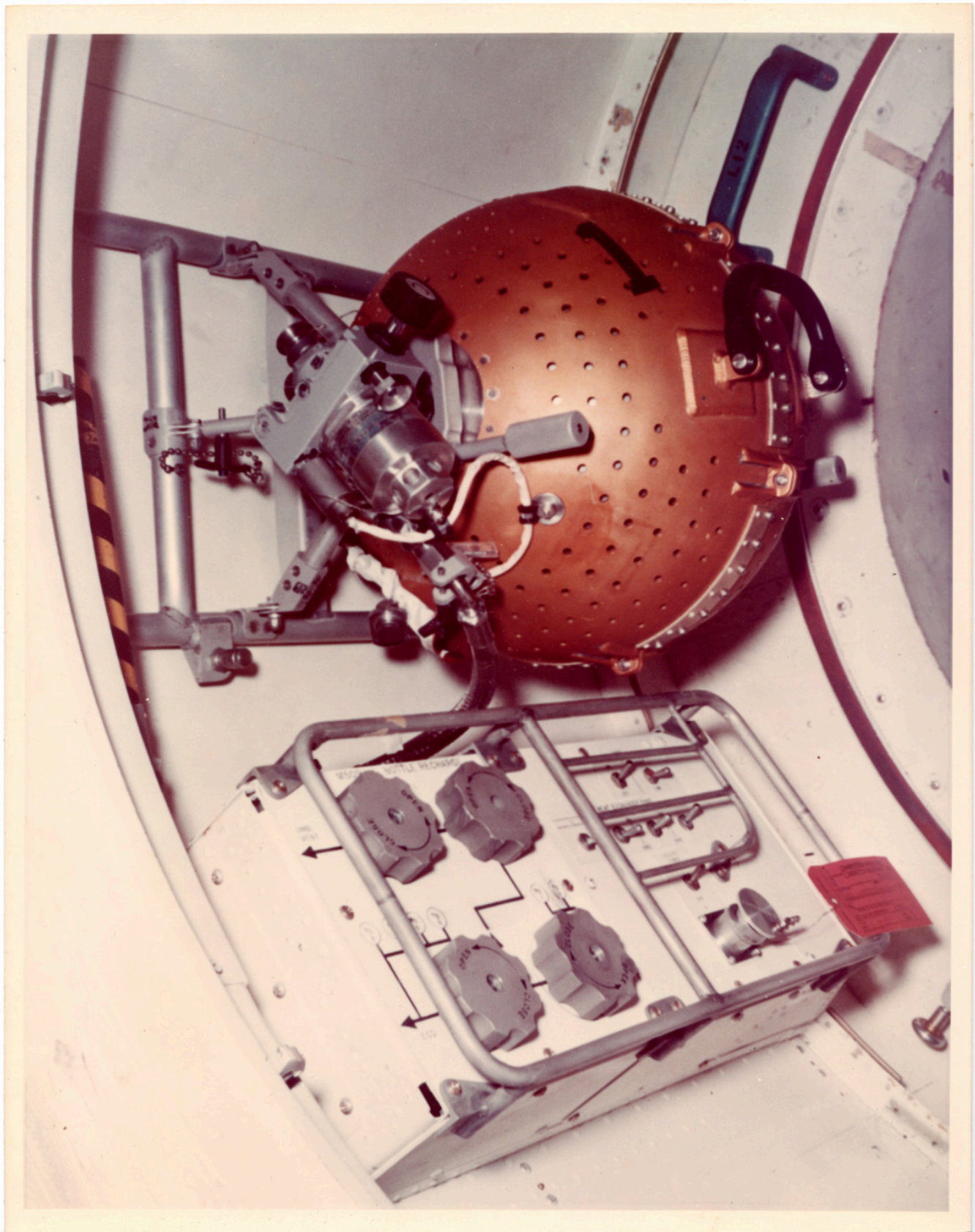
There is a still caption on the back which reads: "AIRLOCK NASA TRAINER ON PRODUCTION LINE IN MDAC-EAST BLDG. -101 FIT CHECK OF EXPERIMENT M509 N2 PRESSURE BOTTLE., NASA-1326. INPUT FOR AUG 1971"
