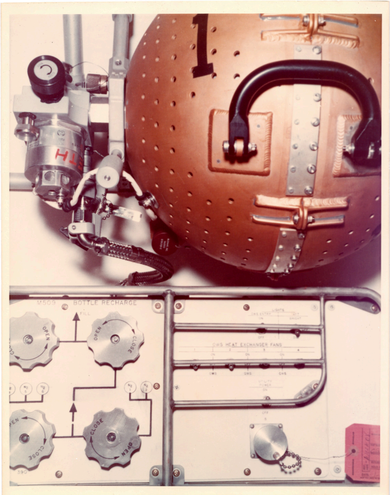
There is a still caption on the back which reads: "AIRLOCK NASA TRAINER ON PRODUCTION LINE IN MDAC-EAST BLDG. -101 FIT CHECK OF EXPERIMENT M509 N2 PRESSURE BOTTLE HOSE ATTACHED TO NIPPLE."
