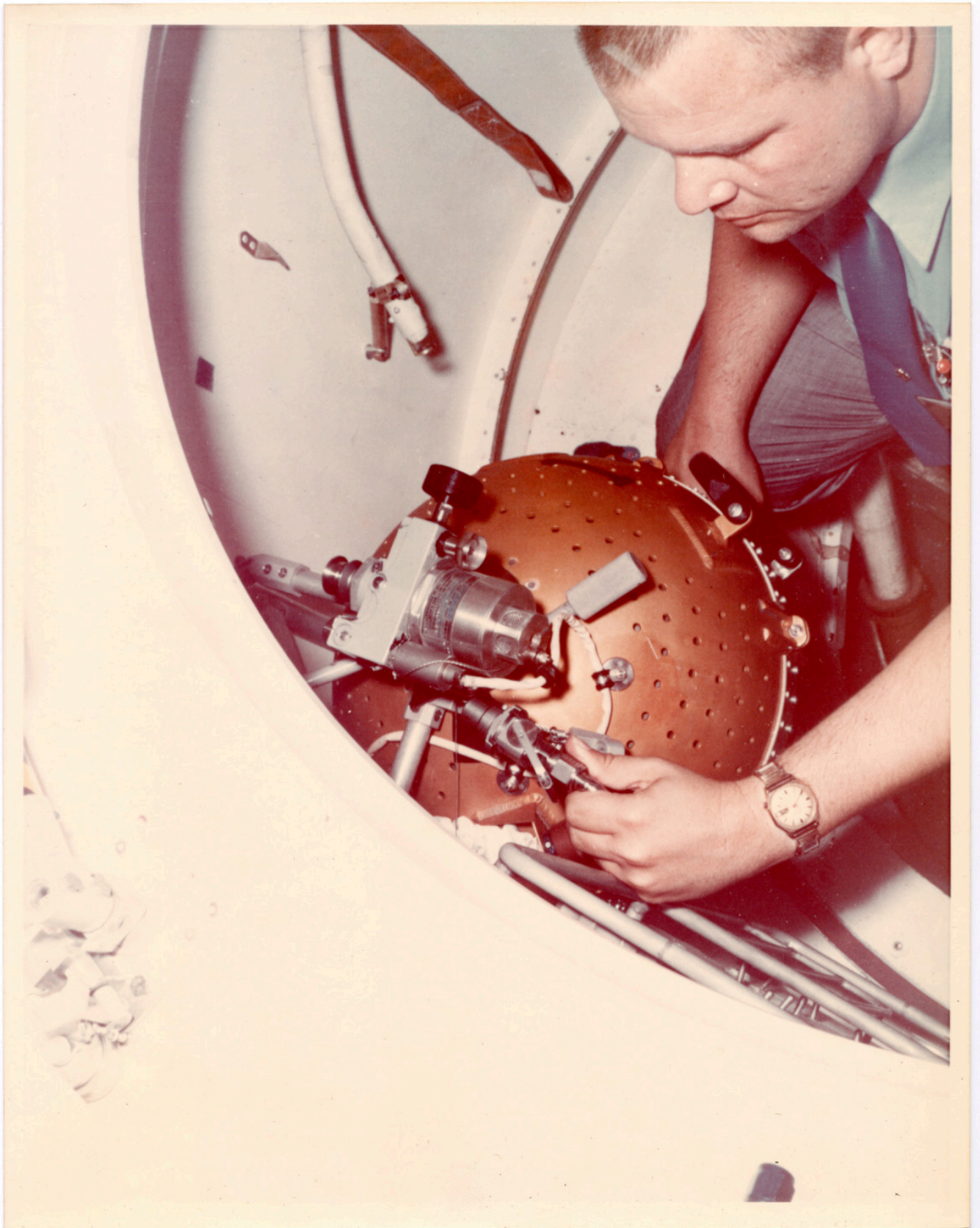
There is a still caption on the back which reads: "AIRLOCK NASA TRAINER ON PRODUCTION LINE IN MDAC-EAST BLDG-101, FIT CHECK OF EXPERIMENT M509 ATTACHMENT OF RECHARGE STATION COUPLER TO NIPPLE. NASA-1330, AUG 1971 INPUT."
