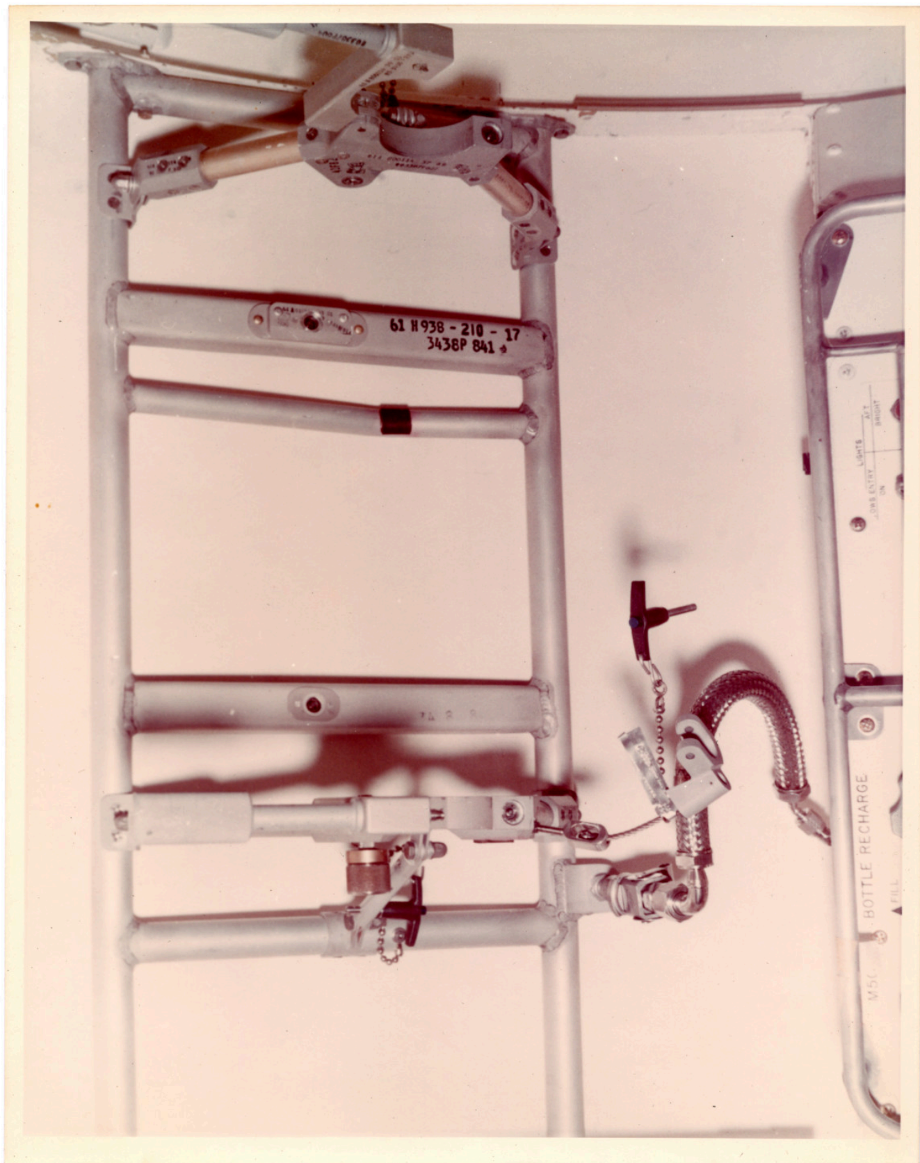
There is a still caption on the back which reads: "AIRLOCK NASA TRAINER ON PRODUCTION LINE IN MDAC-EAST BLDG-101, TRIAL FIT OF EXPERIMENT M-509, RE-CHARGE STATION BRACKET IN POSITION. NASA-1329, AUG. INPUT 1971."
