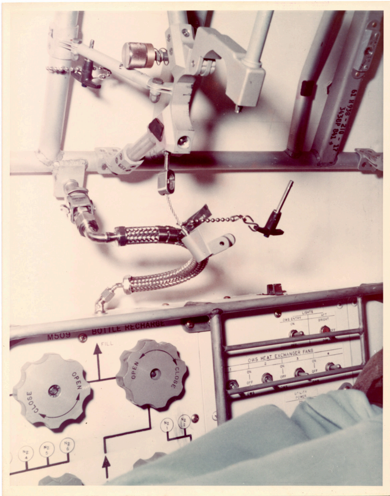
There is a still caption on the back which reads: "AIRLOCK NASA TRAINER ON PRODUCTION LINE IN MDAC-EAST BLDG. -101 FIT CHECK OF EXPERIMENT M-509 RECHARGE STATION HIGH PRESSURE HOSE ATTACHED TO STORAGE NIPPLE. AUG. 1971 INPUT."
