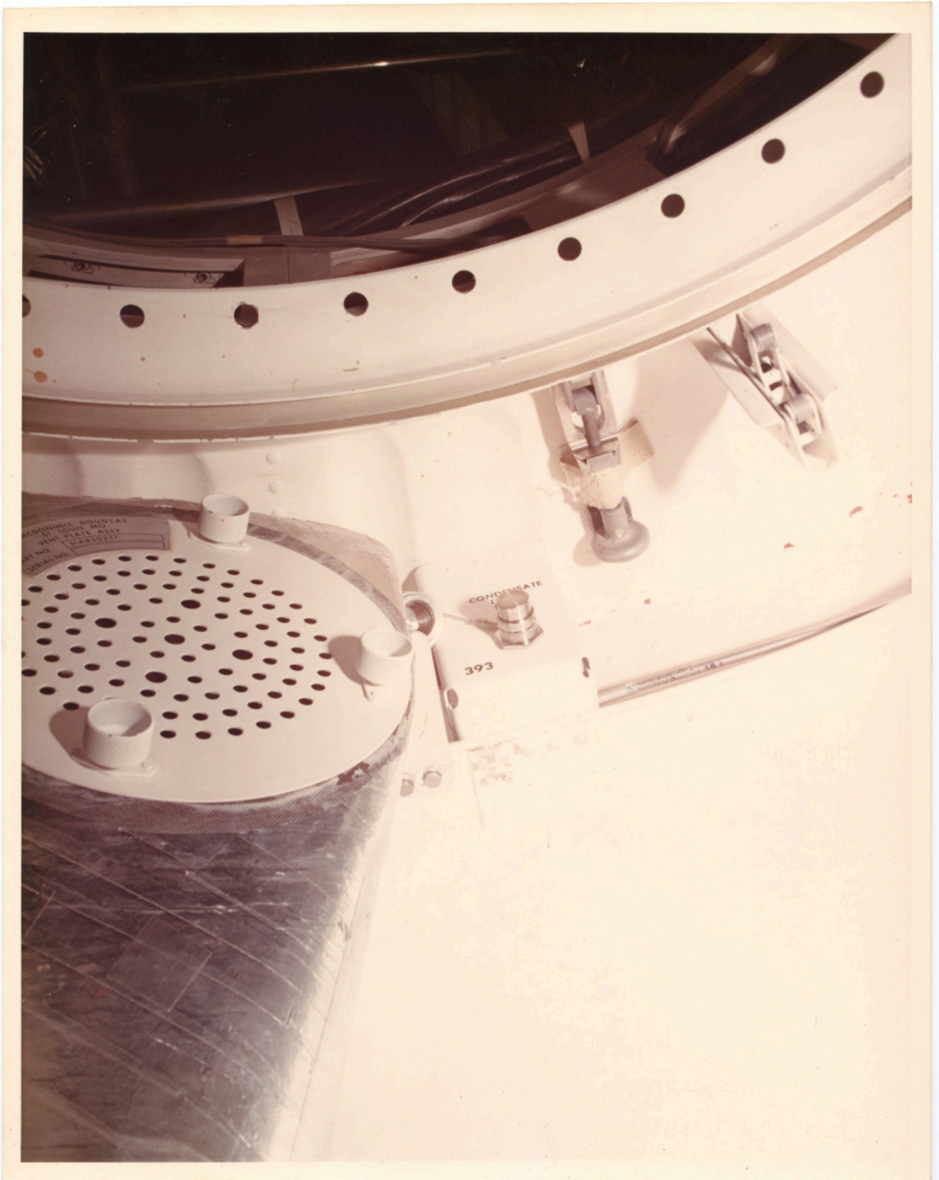
There is a still caption on the back which reads: "Airlock zone 4 closeup of condensate dump port 393. MDAC Input for June."
