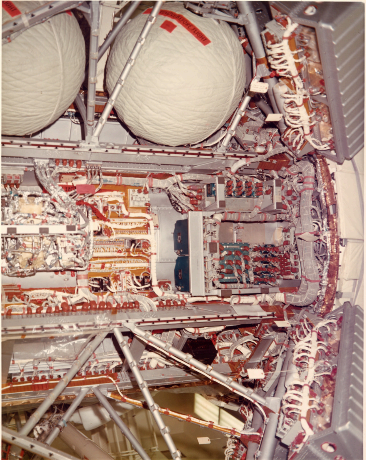
There is a still caption on the back which reads: "AIRLOCK FLIGHT ARTICLE NO. 1 IN CLEAN ROOM. PREPARATION FOR MOVE TO MDAC-E BLDG-66."
