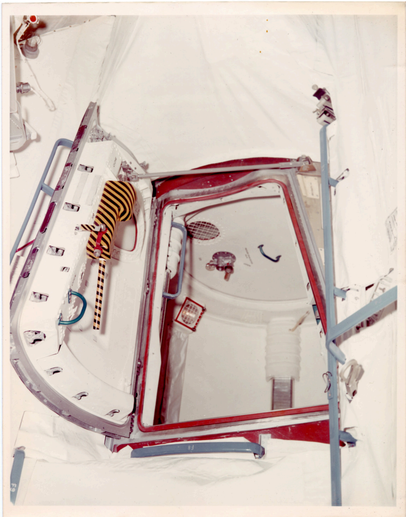
There is a still caption on the back which reads: "NASA-1432, AIRLOCK NASA TRAINER ON PRODUCTION LINE IN MDAC-E BLDG-101 EVA HATCH LOOKING FROM EVA AREA INTO AM LOCK COMPARTMENT."
