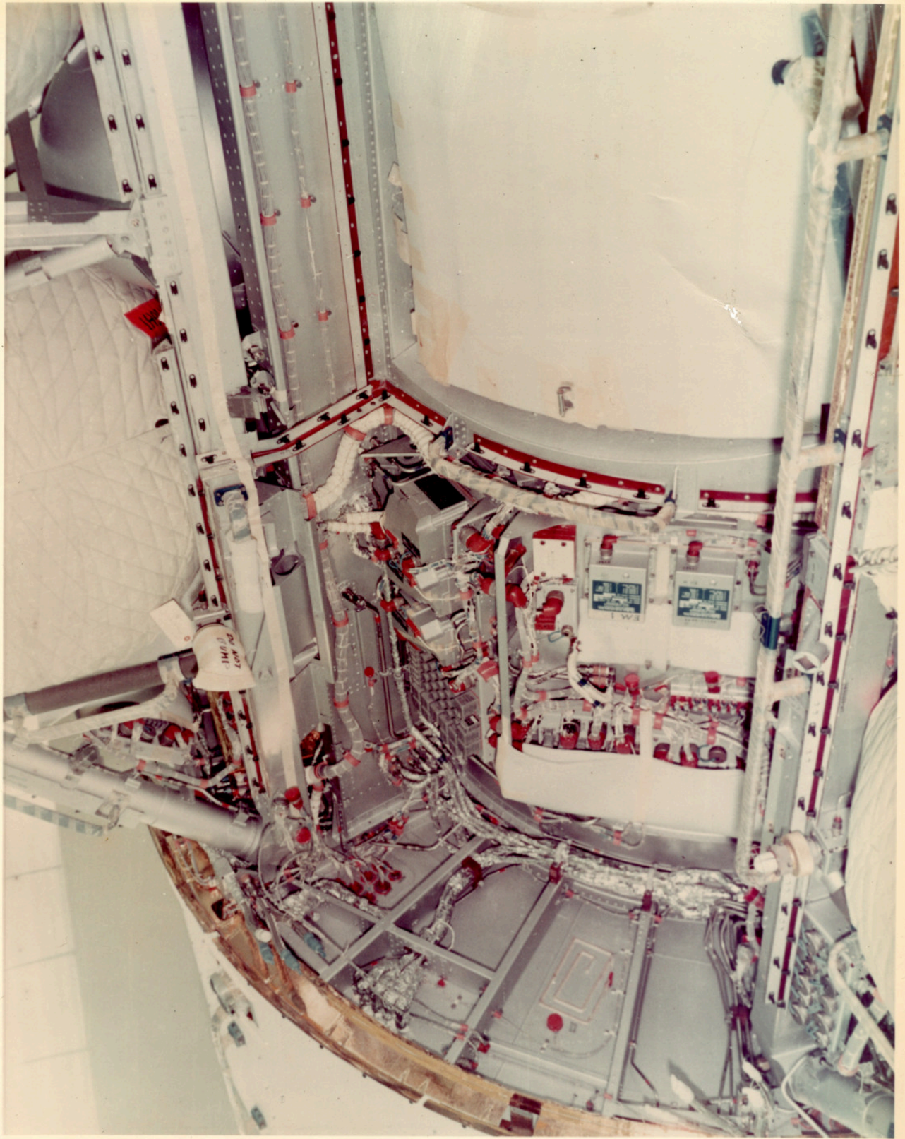
There is a still caption on the back which reads: "AIRLOCK FLIGHT ARTICLE NO. 1 VIEW OF EM NO. 1 AND EV NO. 4 ABOVE EVA HATCH AND BETWEEN +Y AND -Z TRUSSES. NASA-1749"
