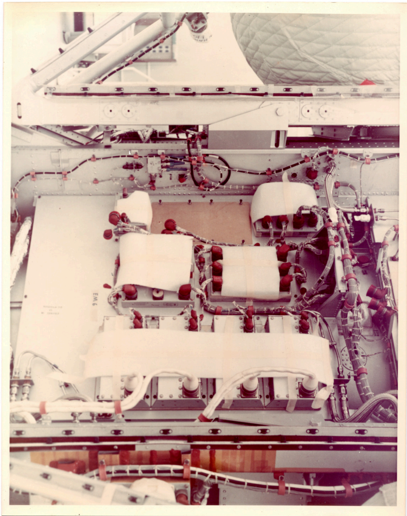
There is a still caption on the back which reads: "AIRLOCK FLIGHT ARTICLE NO. 1 VIEW OF EM NO. 6 LOOKING TOWARD +Y AXIS. NASA-1753."
