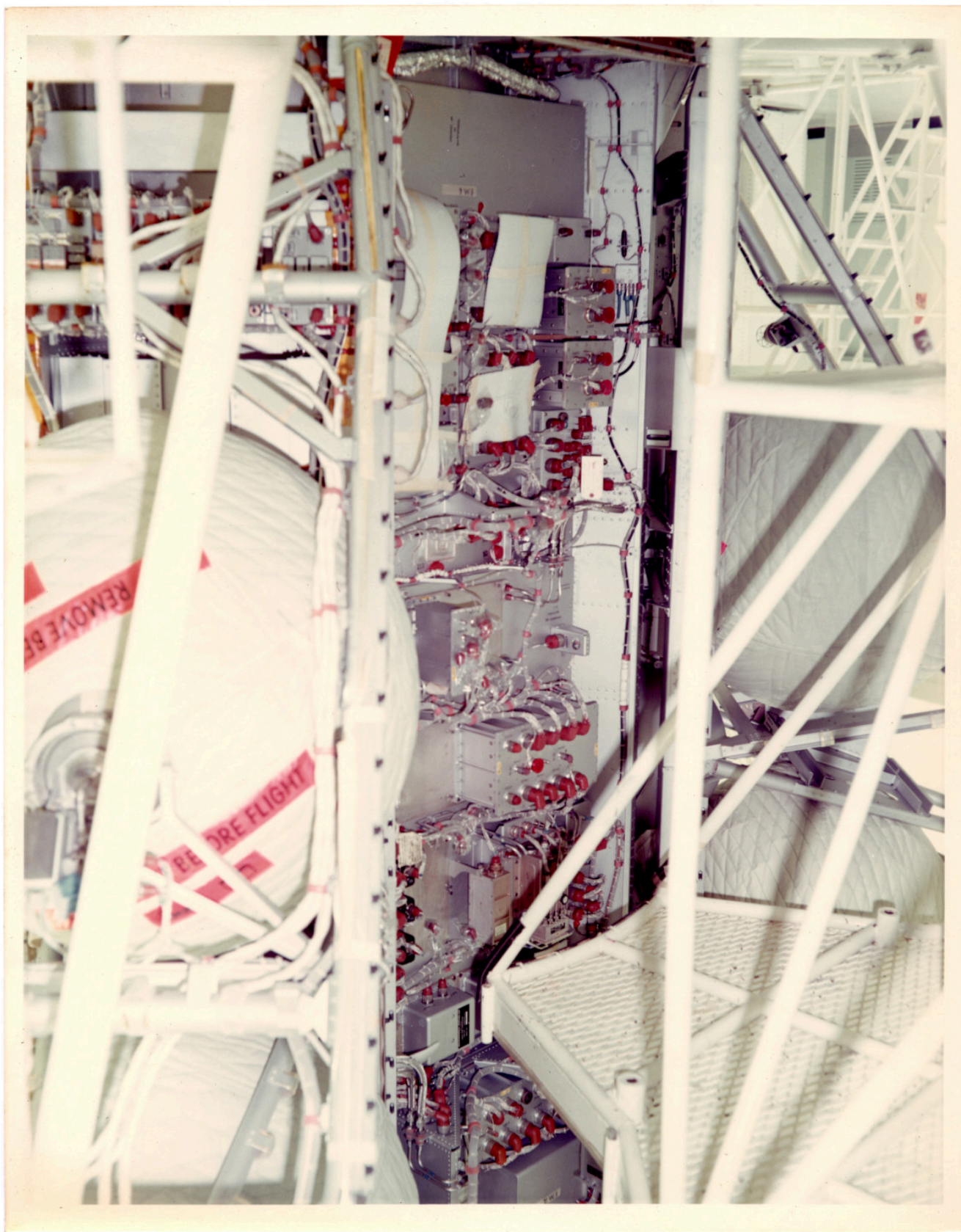
There is a still caption on the back which reads: "AIRLOCK FLIGHT ARTICLE NO. 1 IN CLEAN ROOM AT MDAC-E BLDG-103."
