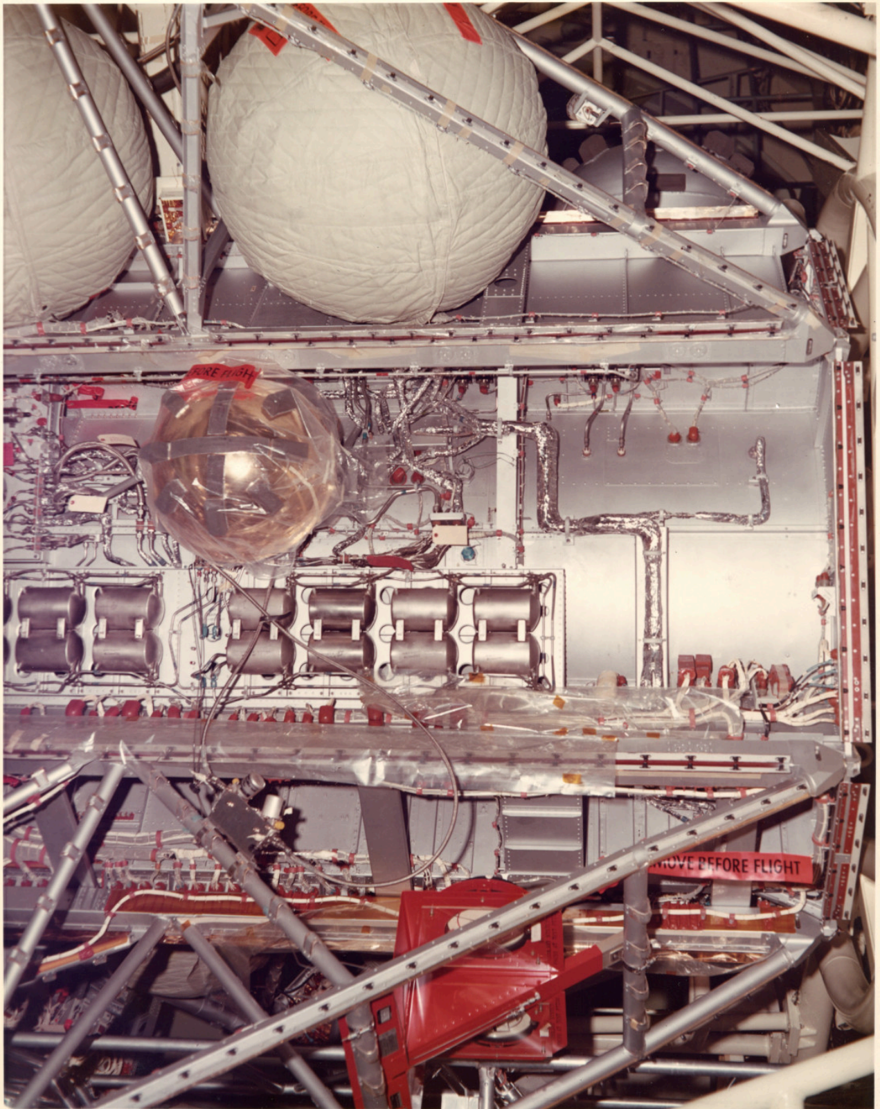
There is a still caption on the back which reads: "AIRLOCK FLIGHT ARTICLE NO. 1 IN CLEAN ROOM. PREPERATION FOR MOVE TO MDAC-E BLDG-66"
