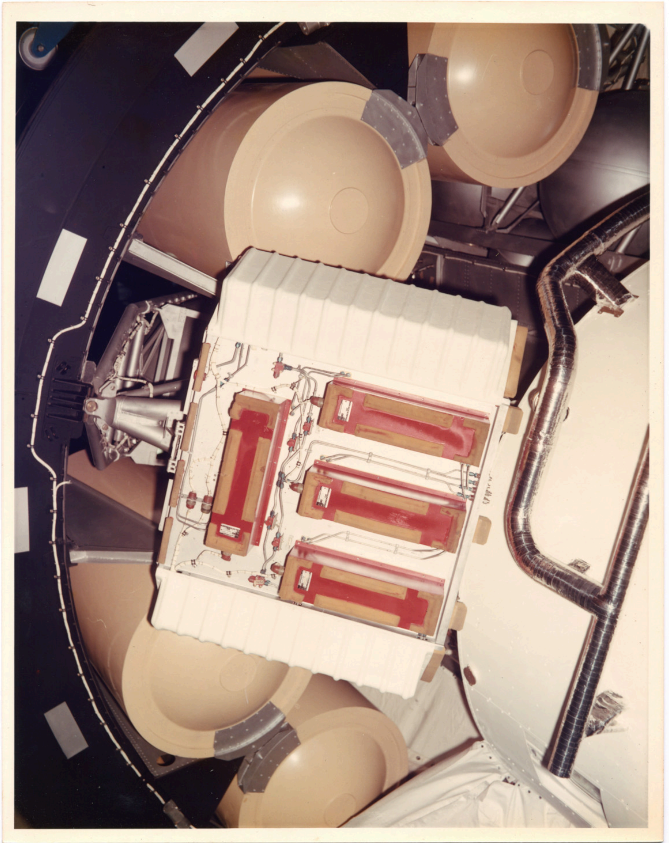
There is a still caption on the back which reads: "NASA-1431, AIRLOCK NASA TRAINER ON PRODUCTION LINE IN MDAC-E BLDG-101 EXTERIOR VIEW SHOWING BATTERY MODULE-1 & N2 TANKS."
