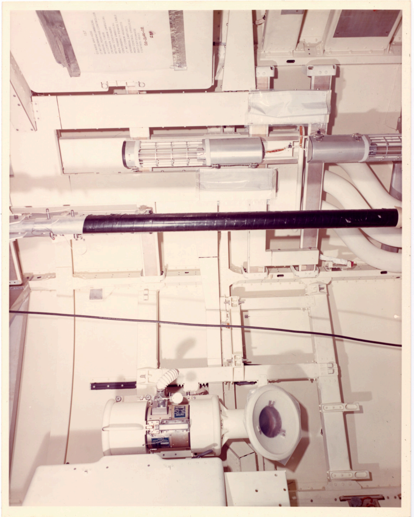
There is a still caption on the back which reads: "INTERIOR VIEW OF LOWER BARREL SECTION SHOWING AREA FAN NO. 2, INTERIOR LIGHTING FIXTURES, CABLE TRAYS. AUG. 1971 INPUT."
