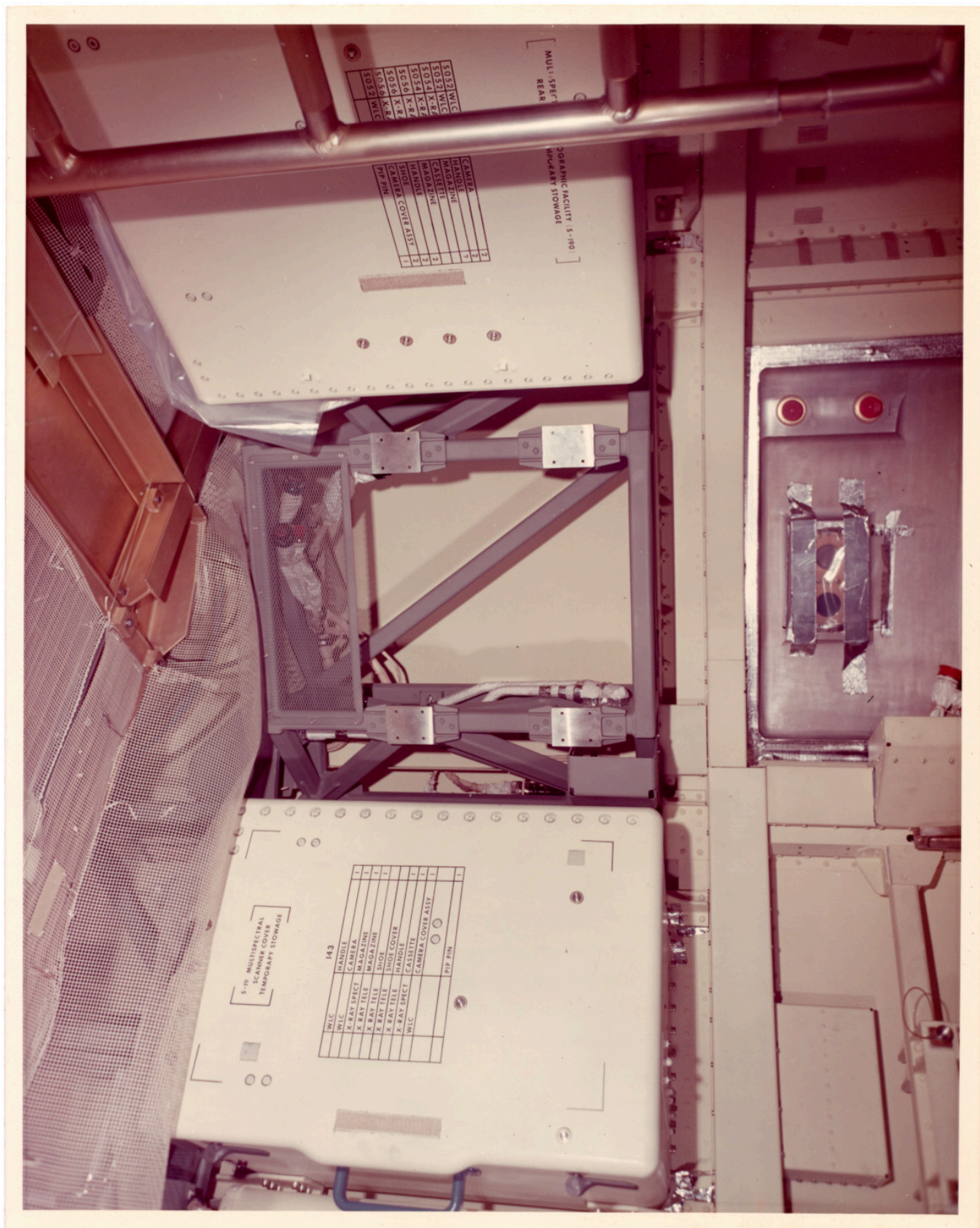
There is a still caption on the back which reads: "MMC MDA Backup Article completed wire bundle installation for Tape Recorder No. 2 and Experiment S192 MDAC Input for month of June."
