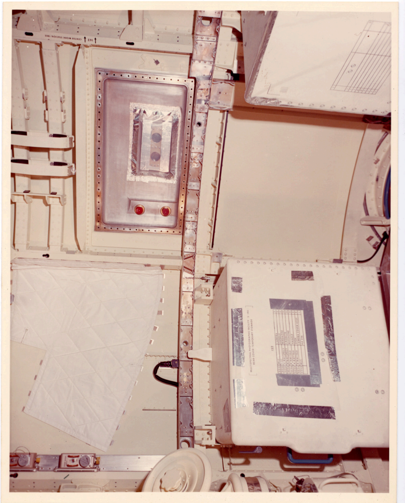
There is a still caption on the back which reads: "MDA BACKUP ARTICLE SHOWING FILM VAULT 2. AND S192 10-BAND SCANNER INSTALLATION AREA."
