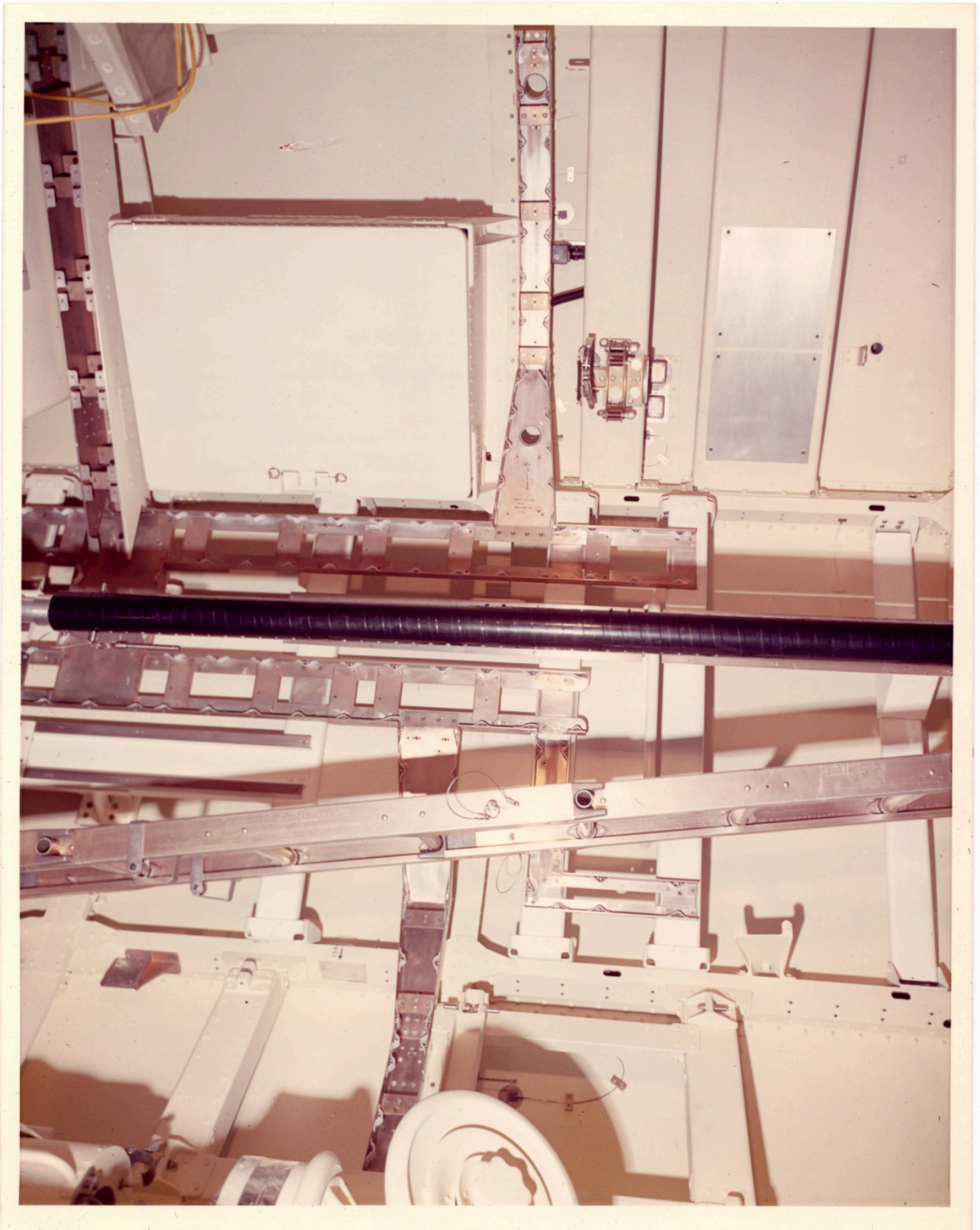
There is a still caption on the back which reads: "MDA BACKUP ARTICLE SHOWING MISCELLANEOUS STOWAGE CONTAINER. FIRE EXTINGUISHER BRACKETRY AND S082 CANISTER INSTALLATION AREA."
