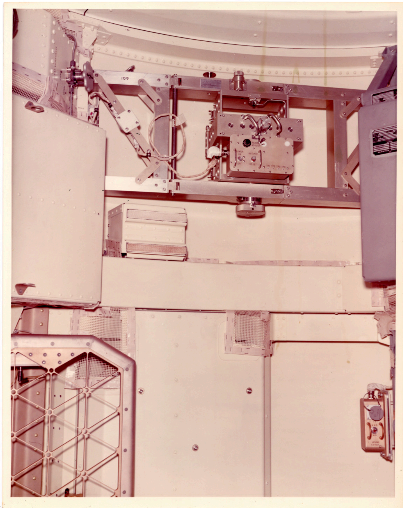
There is a still caption on the back which reads: "AIRLOCK/MDA FLIGHT ARTICLE NO-1 SHOWING S009 AND M512 FOOT RESTRAINT"
