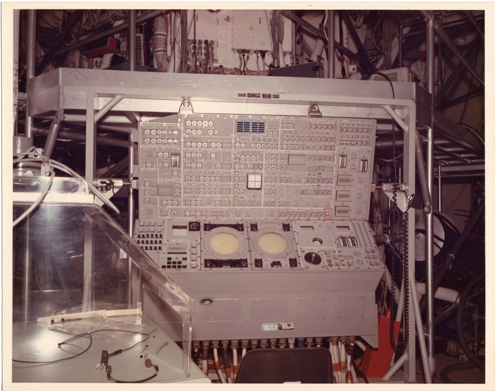
There is a still caption on the back which reads: "ATM Test area in 10K Clean Room Bldg. 4708 front view of C-D panel"
