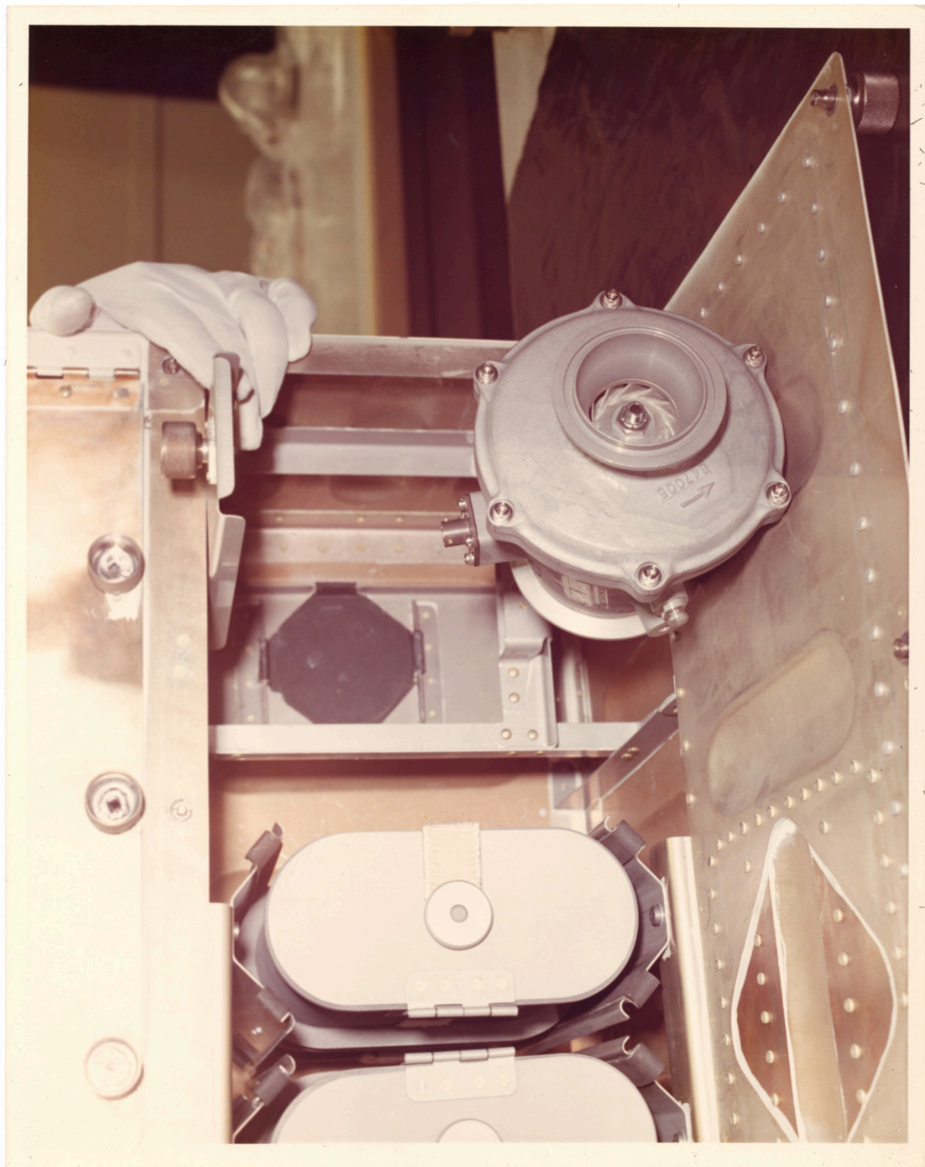
There is a still caption on the back which reads: "Airlock sone 1,11 stowage container. MDAC Input for June."
