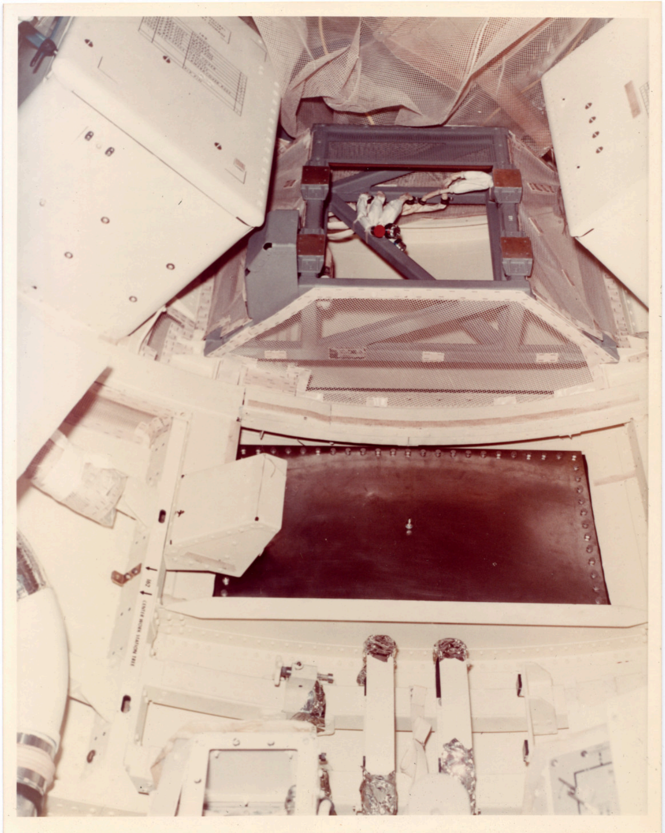
There is a still caption on the back which reads: "AIRLOCK/MDA FLIGHT ARTICLE NO-1 SHOWING 192 BLANKOFF PLATE. FILM VAULT NO-2 & NO-3"
