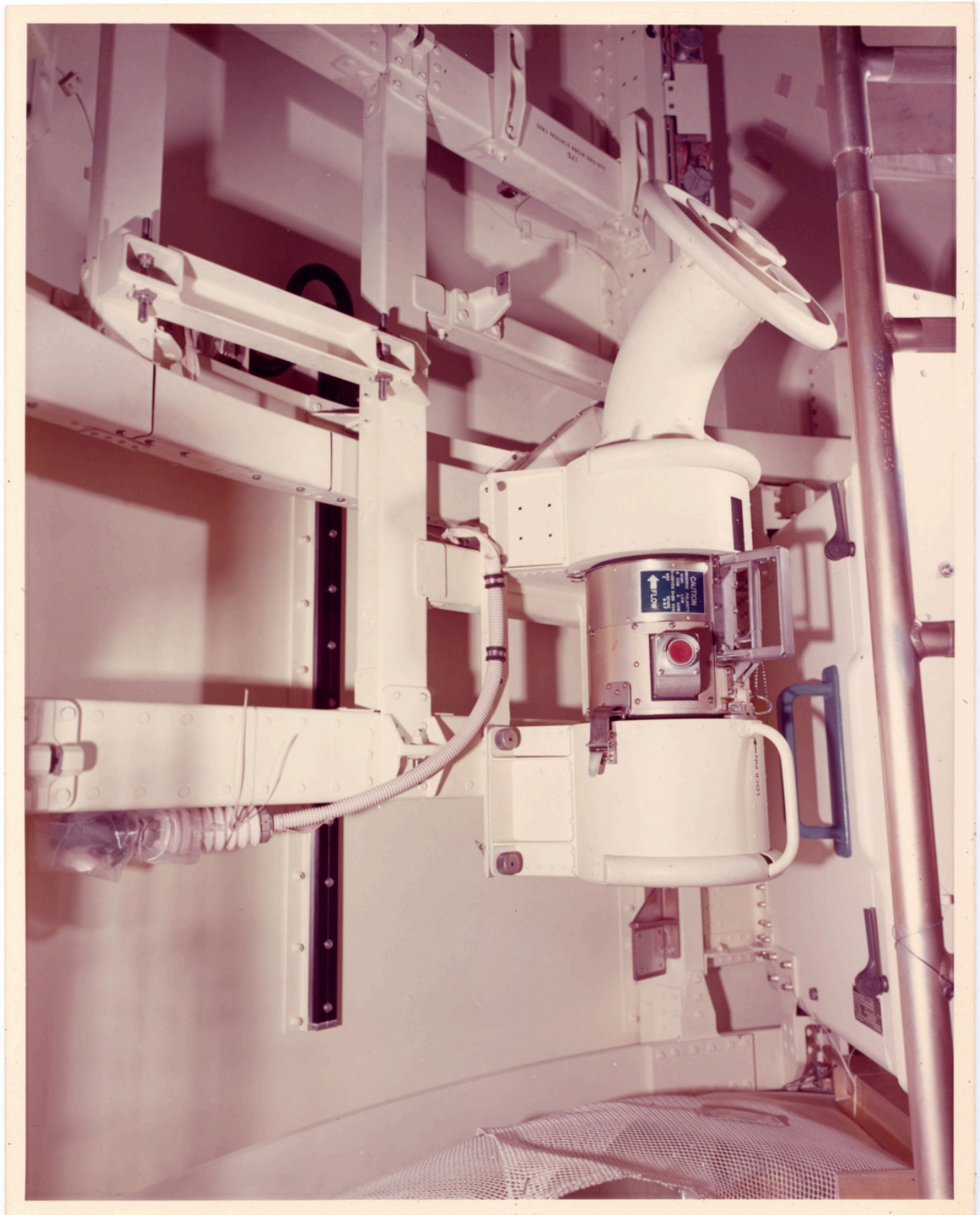
There is a still caption on the back which reads: "INSTALLATION OF CABIN FAN-2 SUN END CASSETTE TREE, AND ASSOCIATED CABLE TRAY COVERS. MDA BACKUP ARTICLE. MDAC INPUT FOR JULY"
