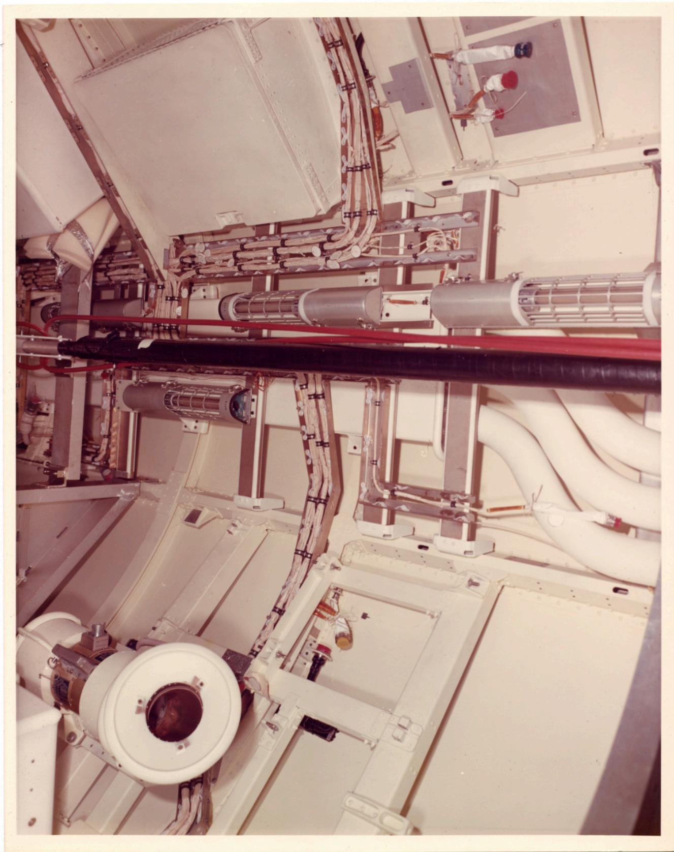
There is a still caption on the back which reads: "MDA Flight Article lower cylinder area showing Fan 7 Muffler Ass'y #2. ECS Duct and Interior Light Fixture, Jul. Input." There is black ink writing on the back which reads: "MFIM"
