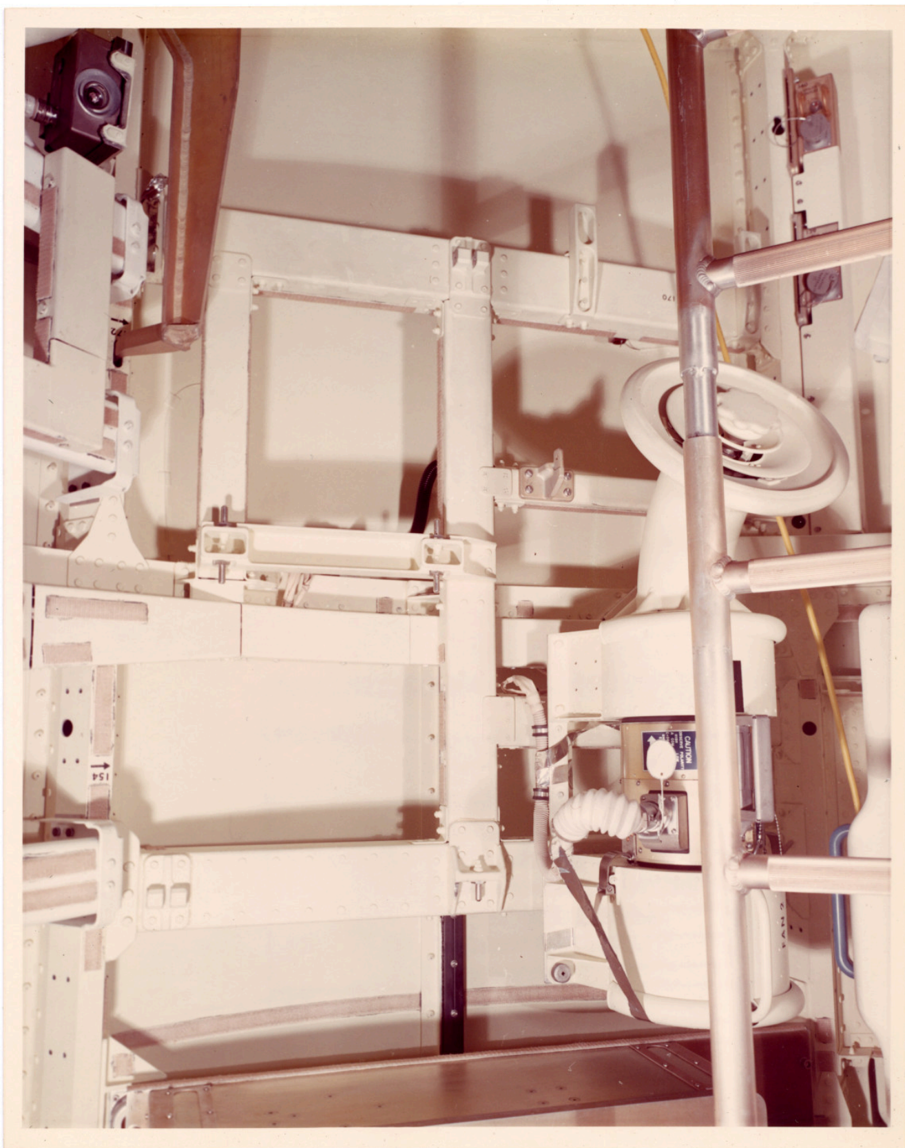
There is a still caption on the back which reads: "INTERIOR VIEW OF THE FLIGHT ARTICLE SHOWING FAN & MUFFLER INSTALLATION AN ULTRAVIOLET FIRE SENSOR APPEARS AT LOWER RIGHT."
