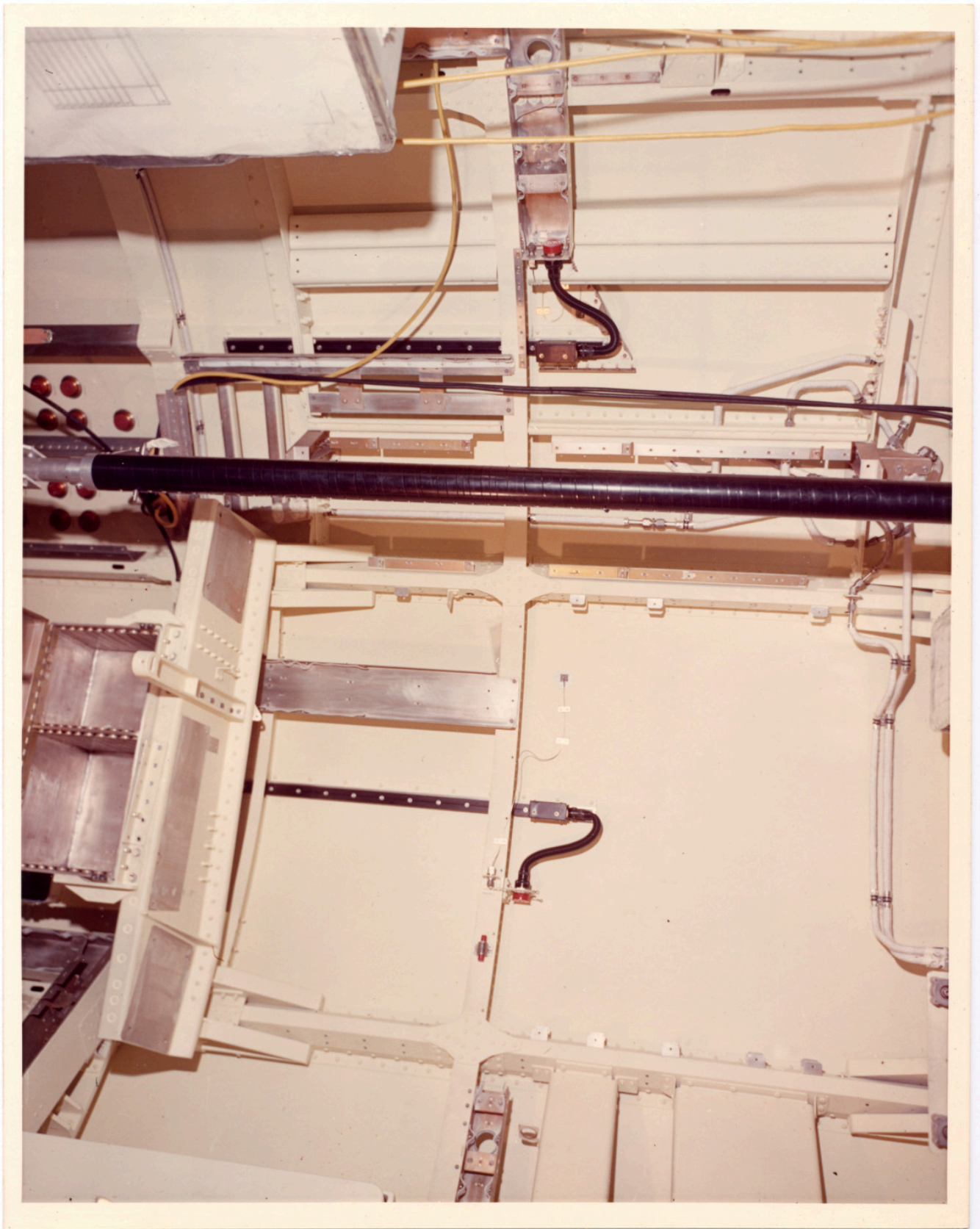
There is a still caption on the back which reads: "MDA BACKUP ARTICLE SHOWING FLIGHT DATA FILE CONTAINER INSTALLATION AND WALL HEATERS."
