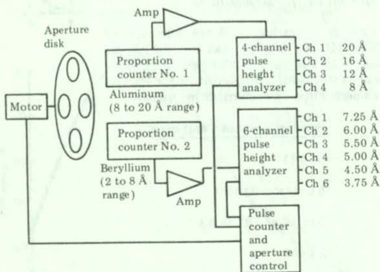
X-ray Event Analyzer
