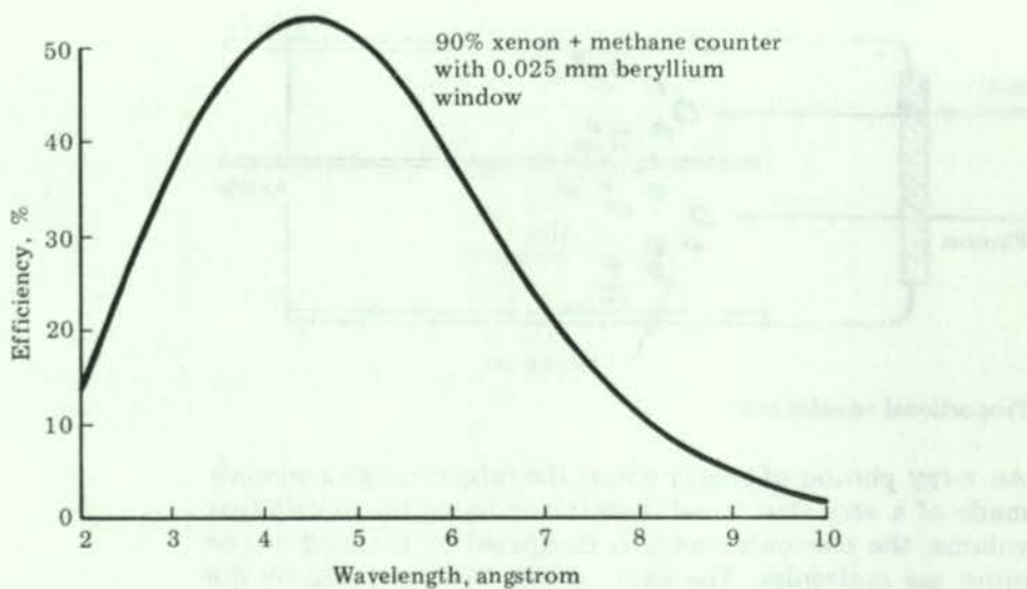
Spectral Response of Aluminum and Beryllium
