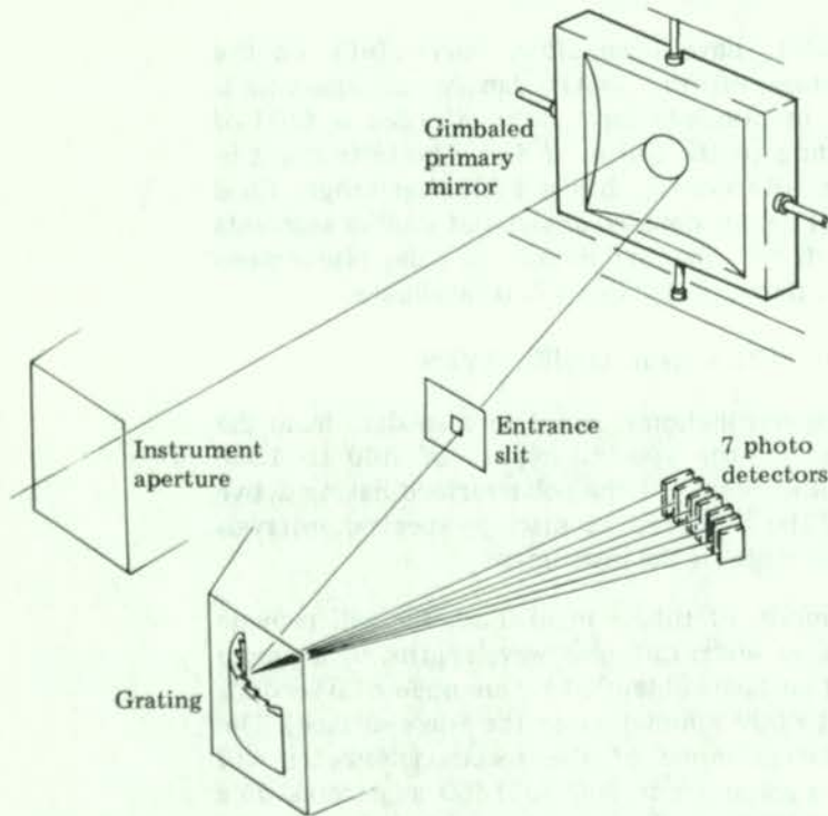
Optical Scheme of Ultraviolet Scanning Polychromator—Spectroheliometer
