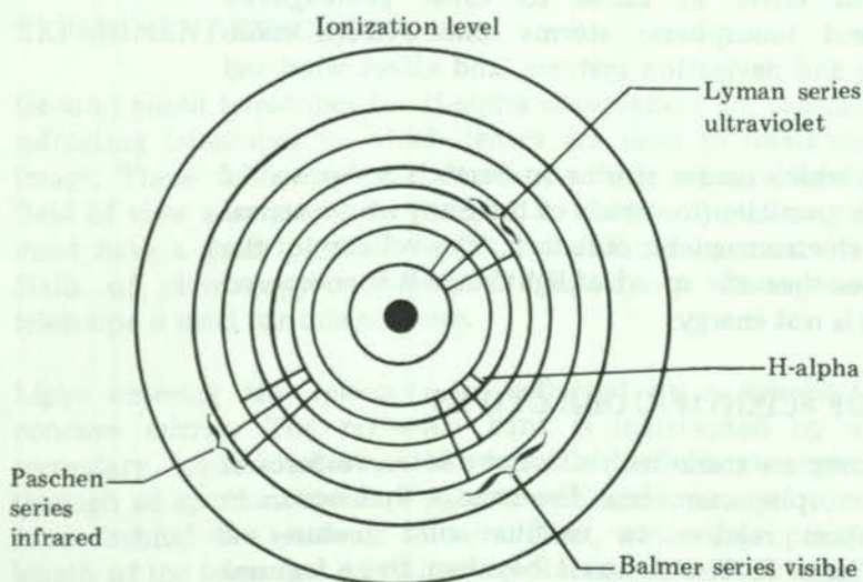
Figure 1 Hydrogen Series
