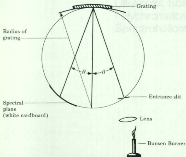
Figure 7 Experiment Layout
