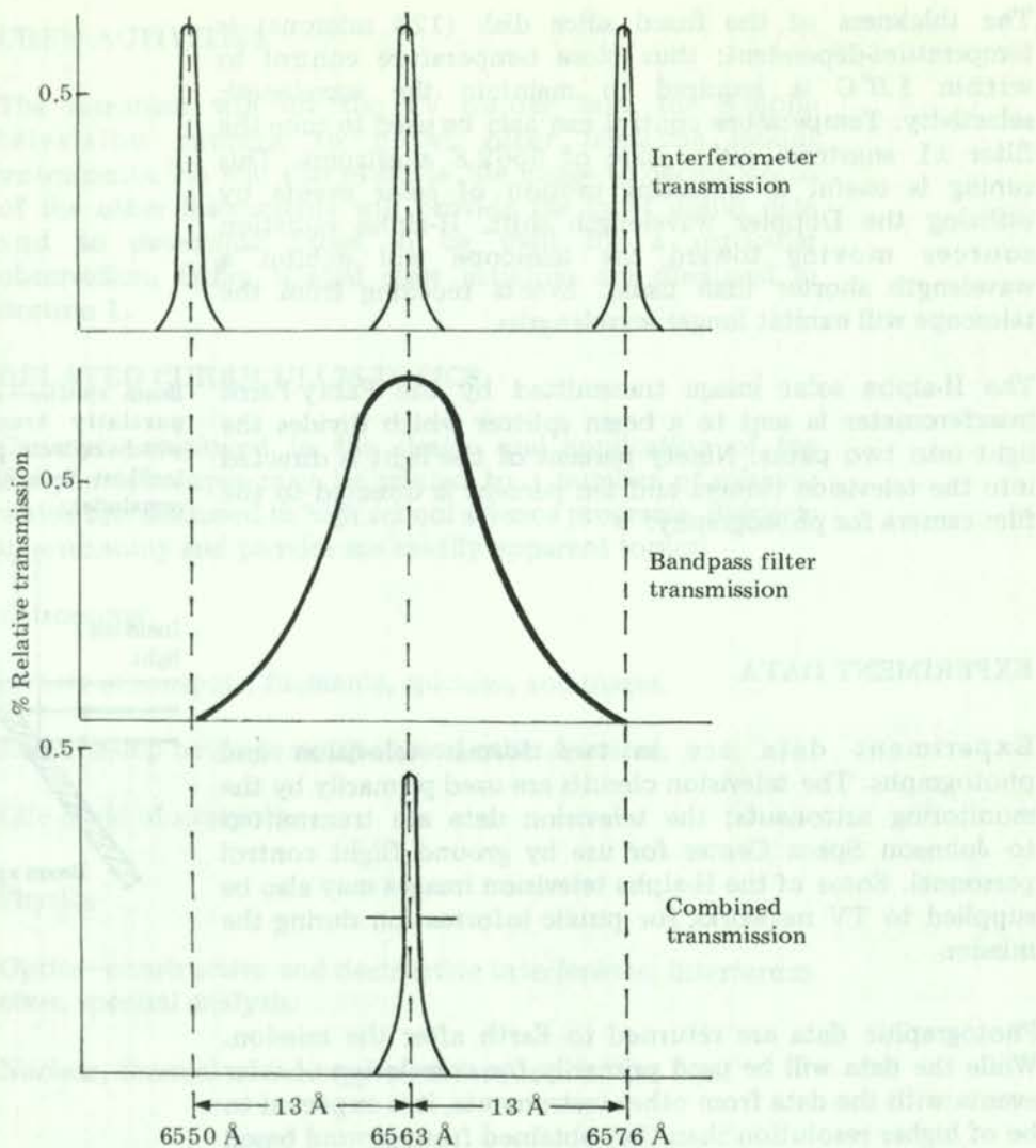
Figure 5 Interferometer Transmission
