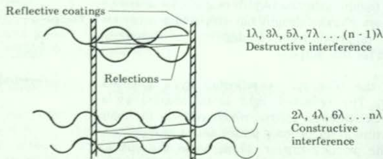
Figure 4 Interferometer Reflections
