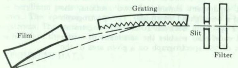
Optical Scheme of Extreme Ultraviolet Spectrograph
