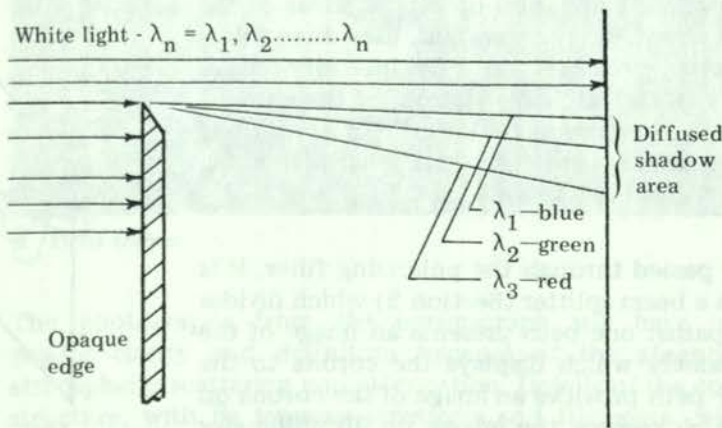
Diffraction of White Light Passing Over an Opaque Edge
