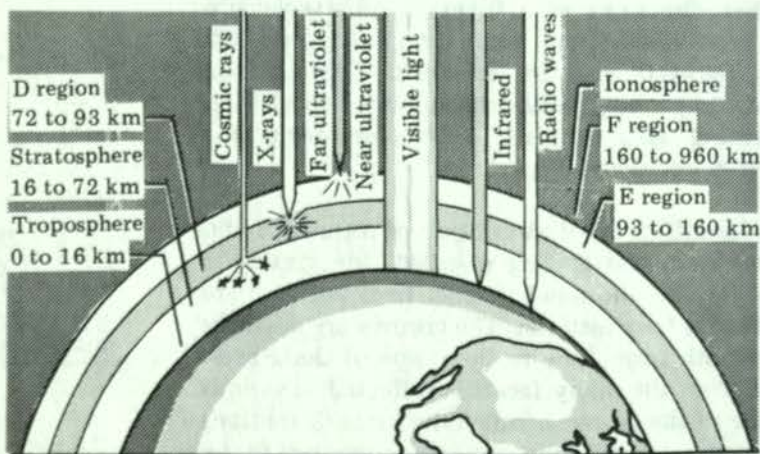
Figure 1 Atmospheric Absorption of Radiation
