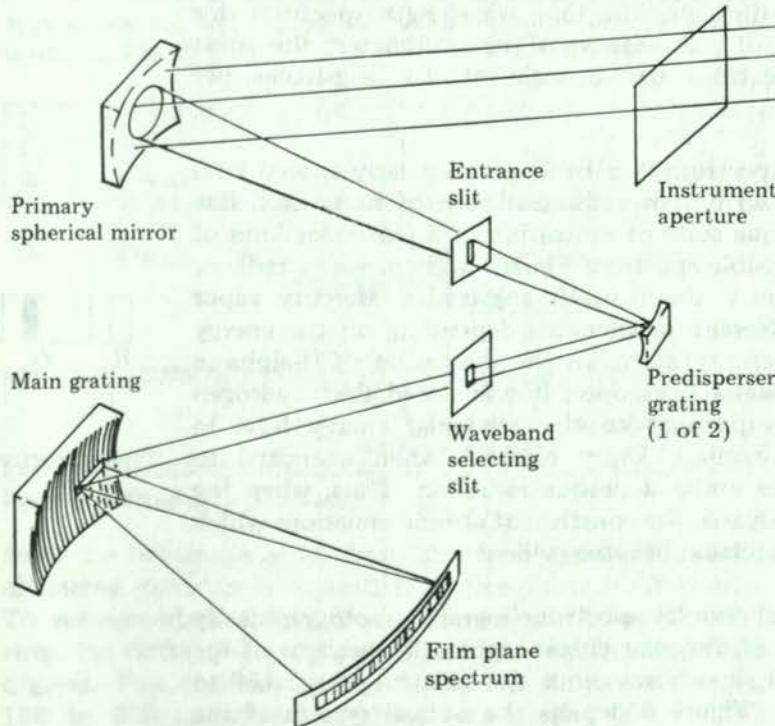
Figure 2 Optical System of the Extreme Ultraviolet Spectrograph
