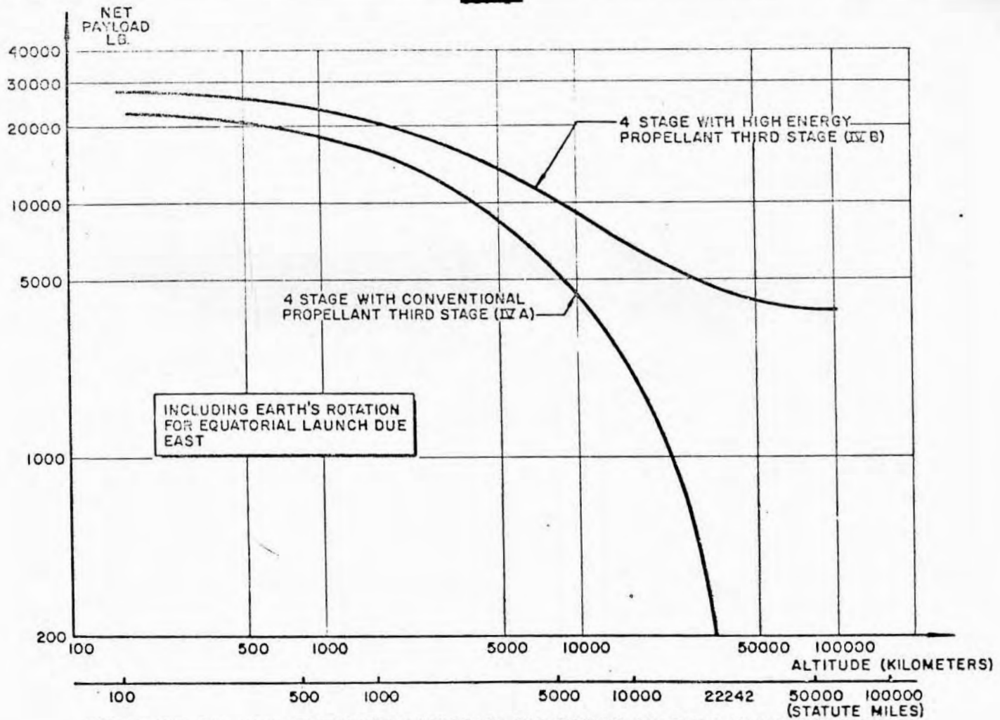
FIG. 13 TYPICAL JUNO V PAYLOAD CAPABILITY FOR ORBITAL MISSIONS (FIRST GENERATION)
