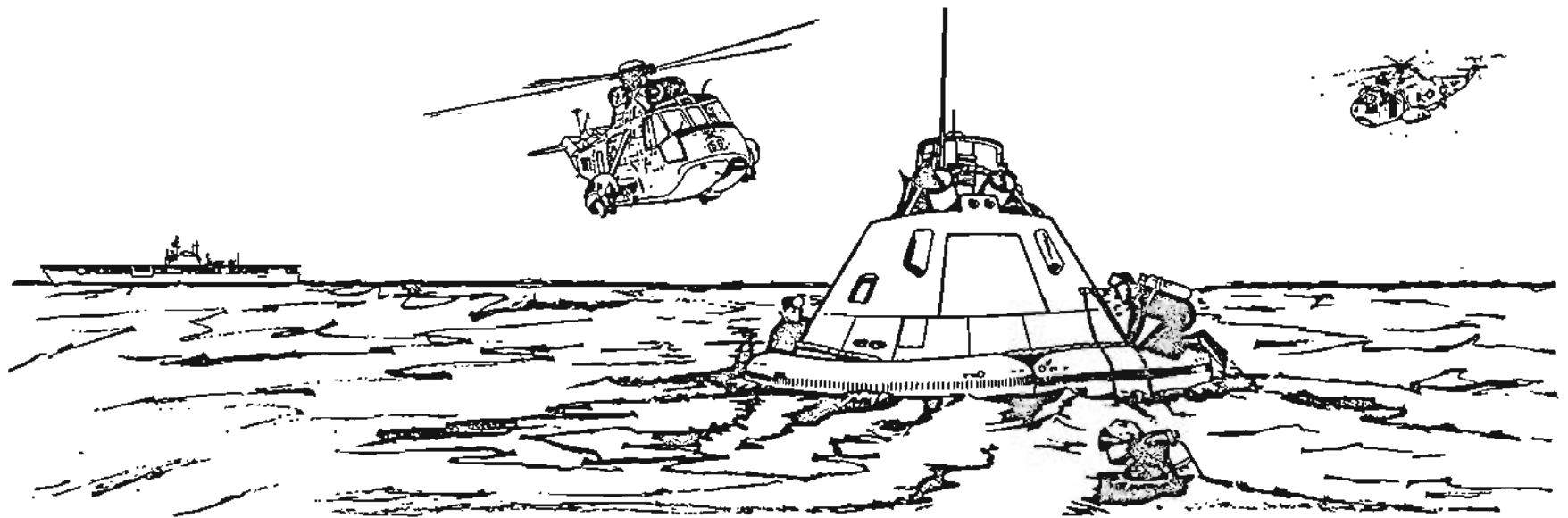
ATLANTIC - SPLASHDOWN
