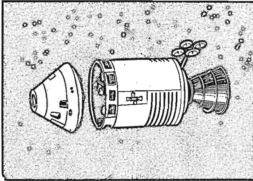
CM/SM SEPARATION
