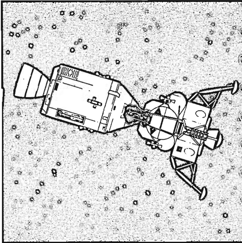
CREW TRANSFER
