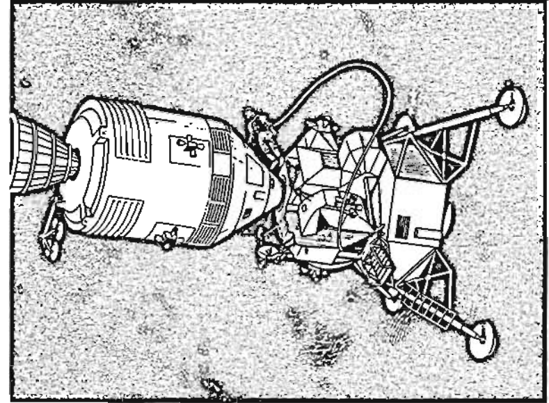
DAY-NIGHT EVA
