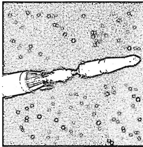
ORBITAL INSERTION
