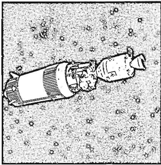
DOCKING
