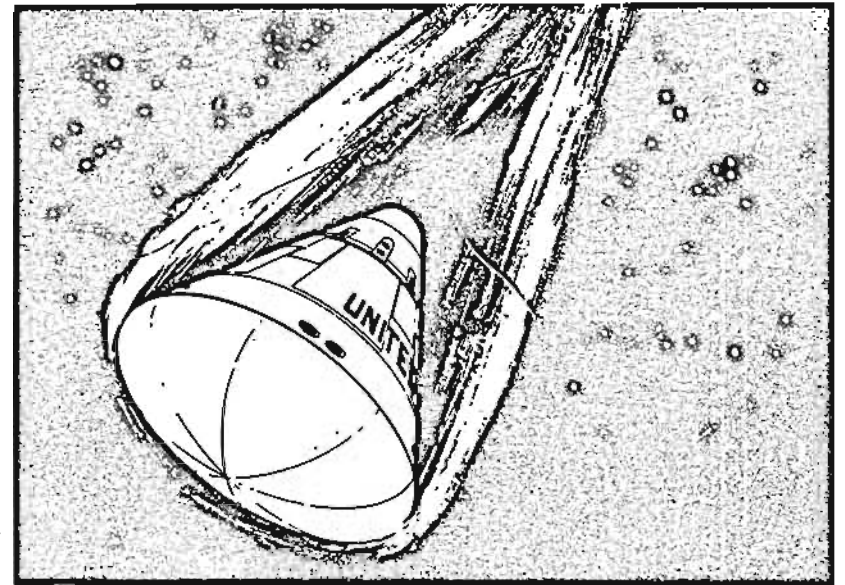
RE-ENTRY
