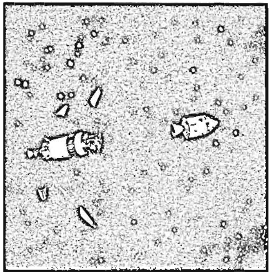
SEPARATION
