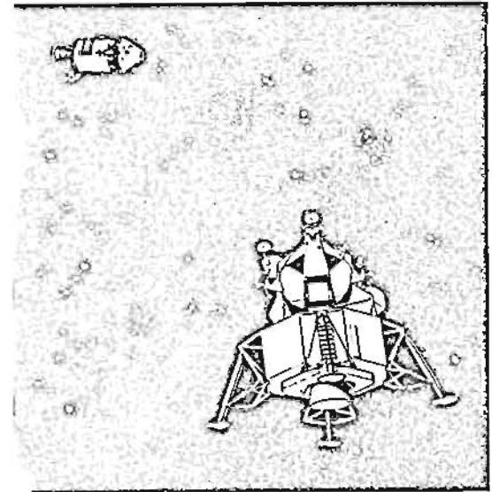
MAXIMUM SEPARATION
