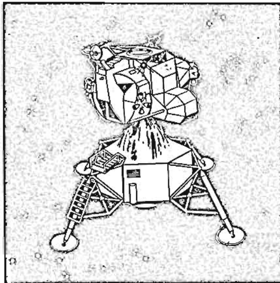
APS BURN
