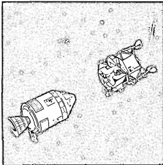
VEHICLES UNDOCKED
