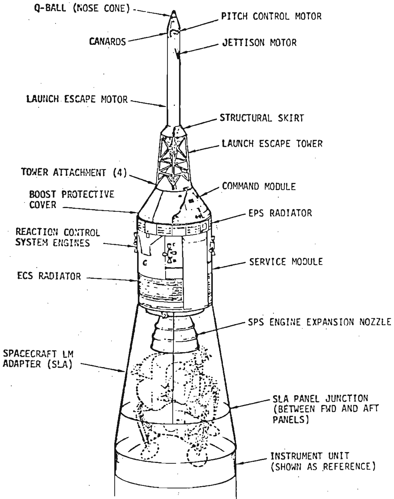
SPACECRAFT CONFIGURATION
