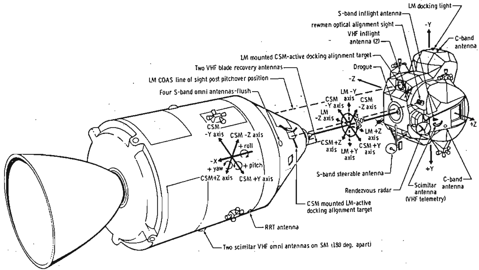
Figure 8-3.2. - LM-CSM antenna locations.
