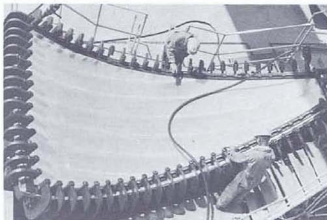
FIGURE 131. EXPLOSIVE FORMING DIES
