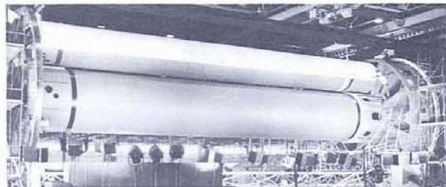
CLUSTERING 70-INCH LOX TANKS
