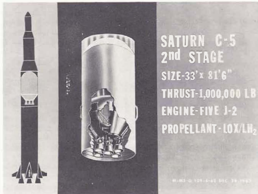
FIGURE 87. S-II STAGE CUTAWAY
