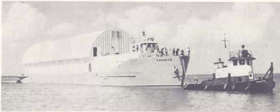
FIGURE 89. BARGE PROMISE
