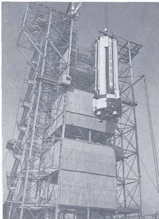
FIGURE 120. SA-D5 BOOSTER
