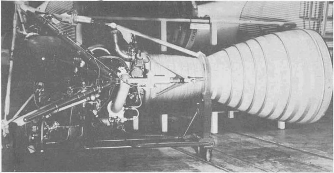
FIGURE 2. THOR-JUPITER ENGINE
