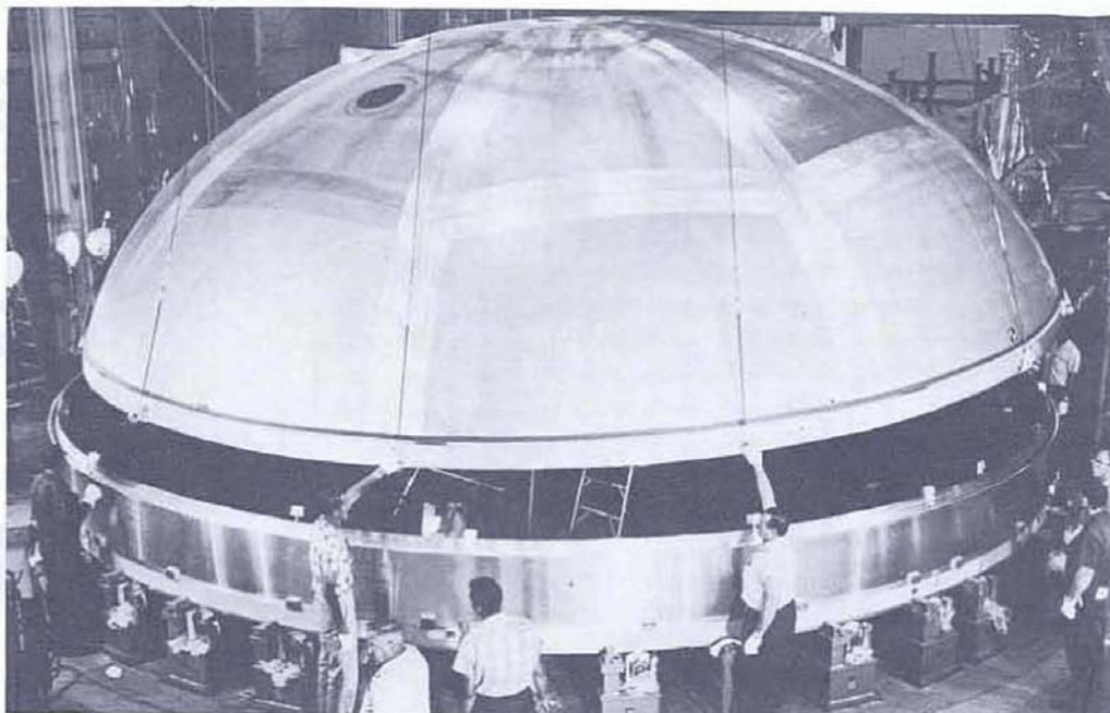
FIGURE 145. MATING BULKHEAD TO Y-RING
