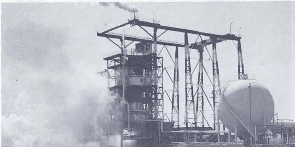
FIGURE 136. COMPLETION OF S-IV BATTLESHIP TEST PROGRAM
