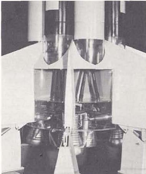
FIGURE 40. REDESIGNED TAIL OF THE SATURN BOOSTER
