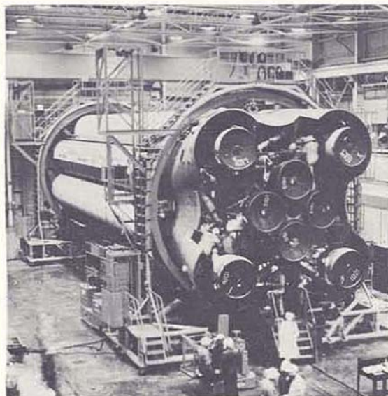
FIGURE 31. FLIGHT BOOSTER CHECKOUT
