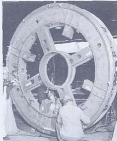
LOWER THRUST RING
