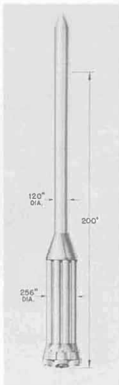
FIGURE 6. SATURN B
