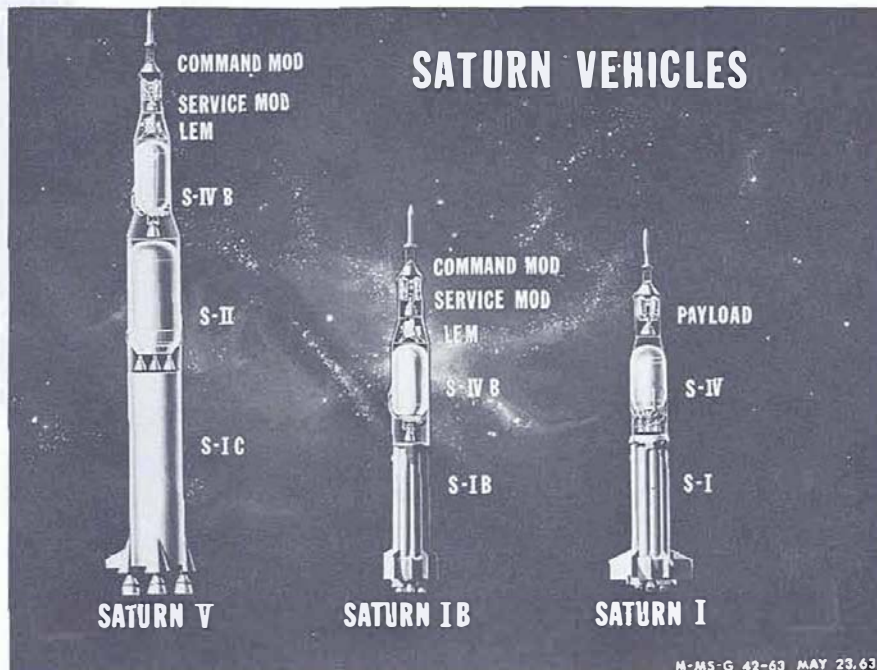
FIGURE 123. SATURN VEHICLES
