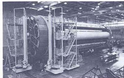
FIGURE 139. FABRICATION AND ASSEMBLY OF S-I-8 AT MICHLOUD
