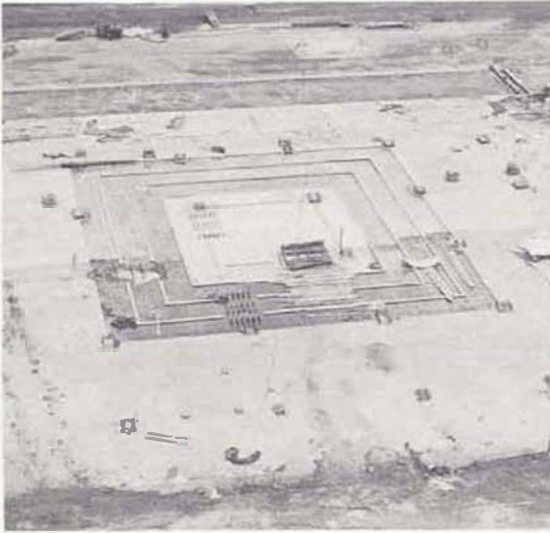
FIGURE 141. SATURN V DYNAMIC TOWER
