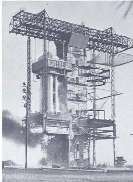
FIGURE 129. STATIC FIRING OF S-I-5
