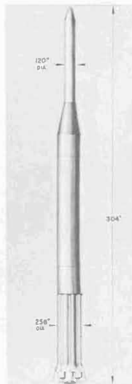
FIGURE 7. SATURN C
