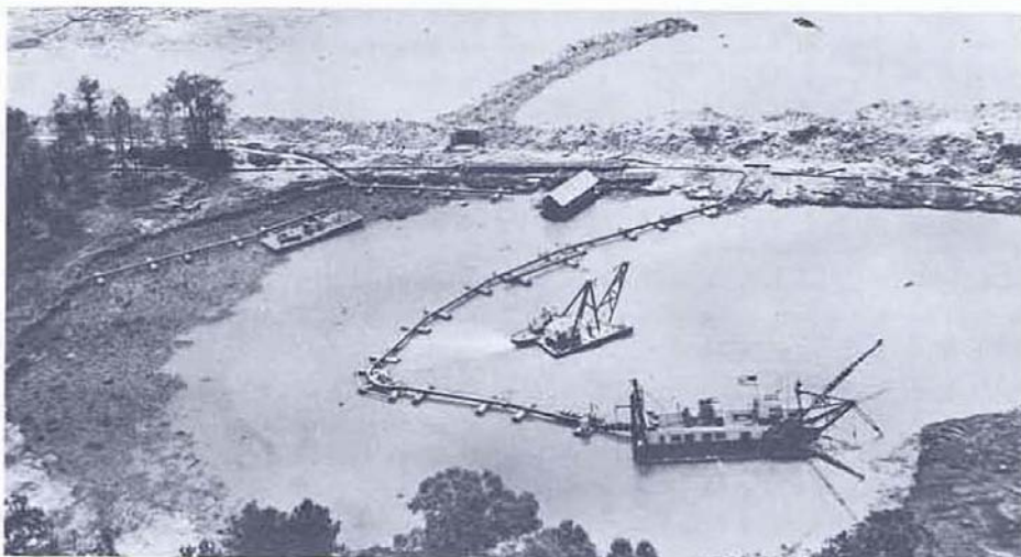
FIGURE 144. DREDGING AT MISSISSIPPI TEST OPERATIONS
