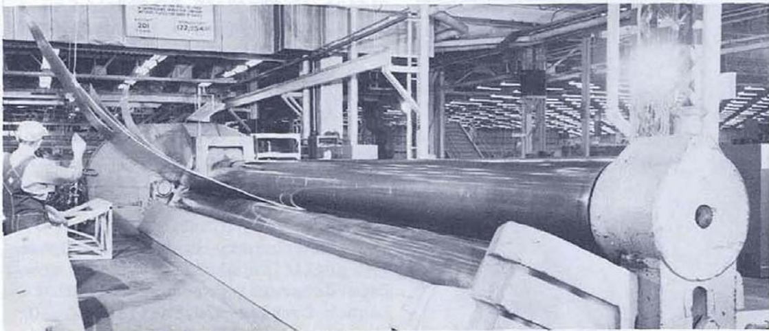
FIGURE 124. S-IC BULKHEAD GORE FORMING
