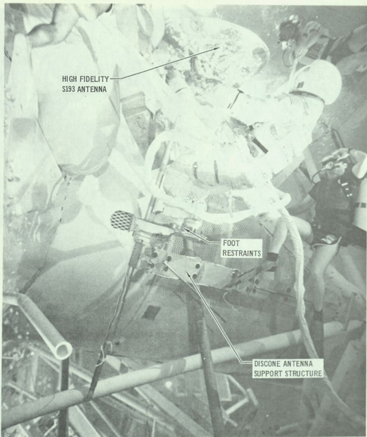
FIGURE 5-45 FOOT RESTRAINT LOCATION FOR S193 REPAIR
