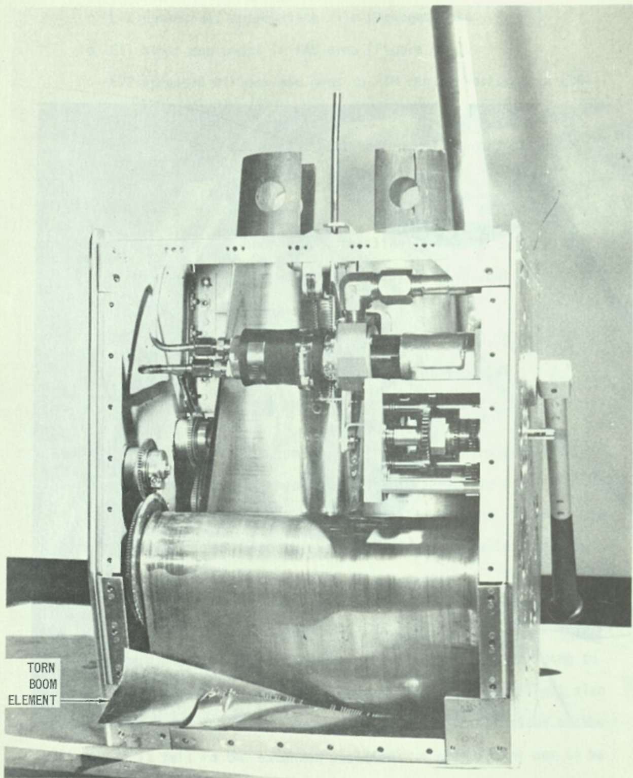
FIGURE 5-3 NBS EXTENSIBLE BOOM (COVER REMOVED)
