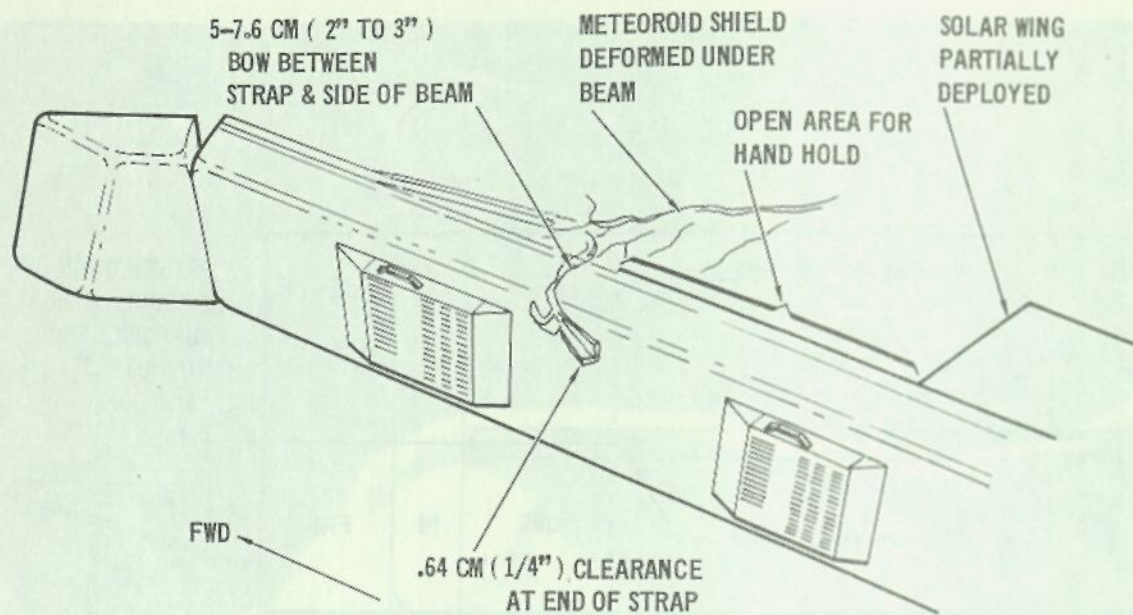
FIGURE 5-24 CONFIGURATION OF SAS WING NO. 1 PER TELECON WITH CREW - CDT 1430 6/1/73
