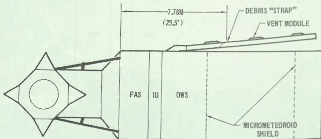
FIGURE 5-25 SAS BEAM DEPLOYMENT AREA
