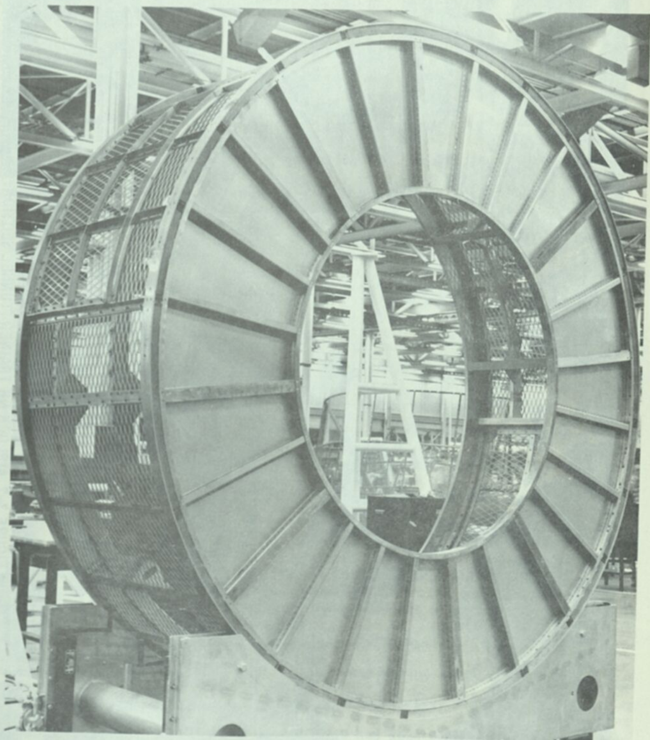
FIGURE 3-3 AIRLOCK STRUCTURAL TRANSITION SECTION (STS) NB TRAINER
