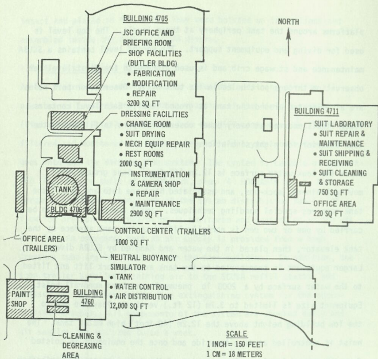
FIGURE 1-2 MSFC NEUTRAL BUOYANCY FACILITIES
