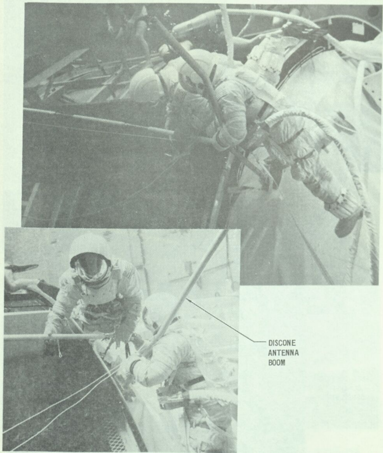
FIGURE 5-32 NBS EXERCISE EVALUATING RESTRAINING METHODS AT THE DISCONE ANTENNA AREA
