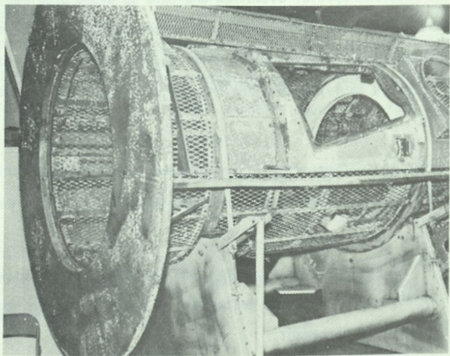
FIGURE 4-2 FASTENER CORROSION
