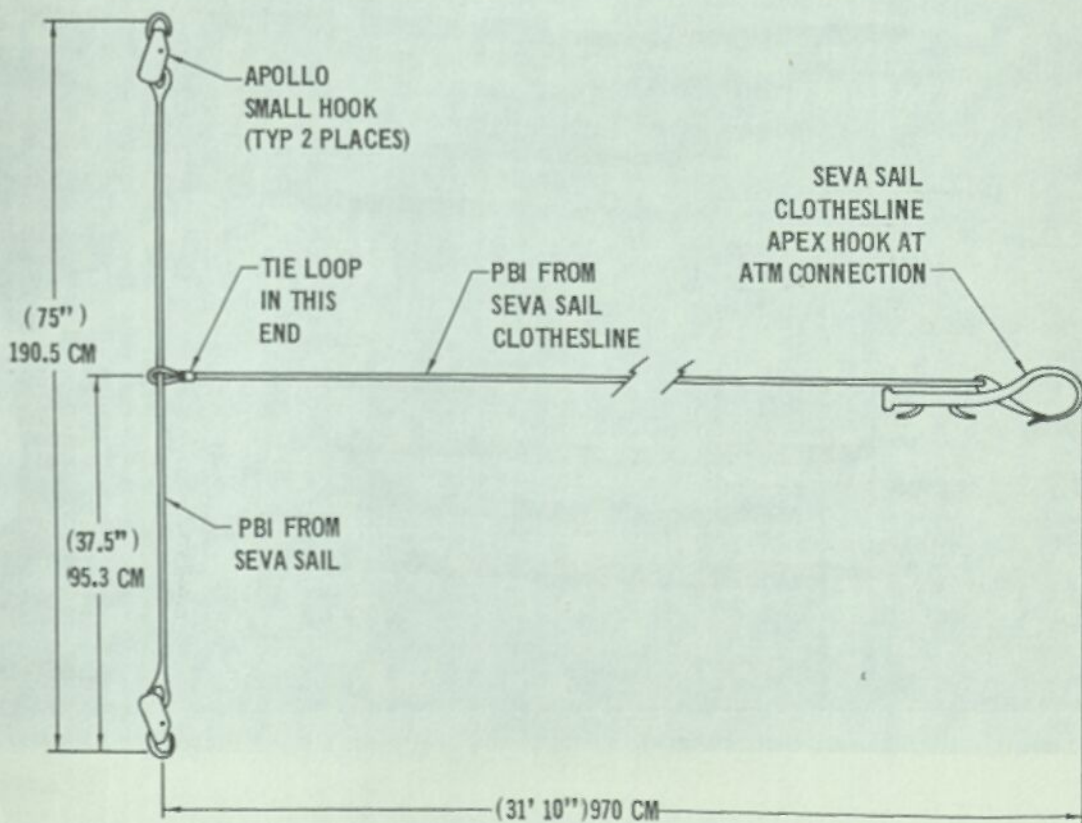
FIGURE 5-38 BOOM ERECTION TETHER (BET) 5-54
