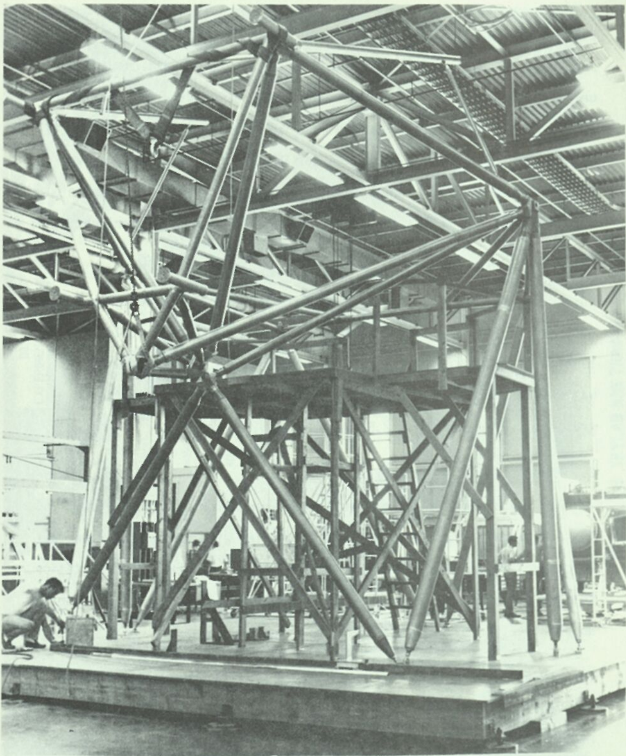
FIGURE 3-7 NBS DEPLOYMENT ASSEMBLY (DA)
