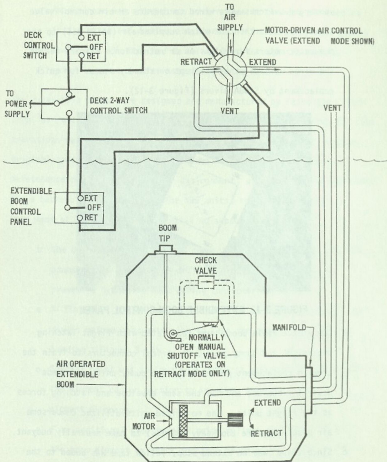
FIGURE 3-11 SCHEMATIC OF NBS AIR OPERATED EXTENDIBLE BOOM
