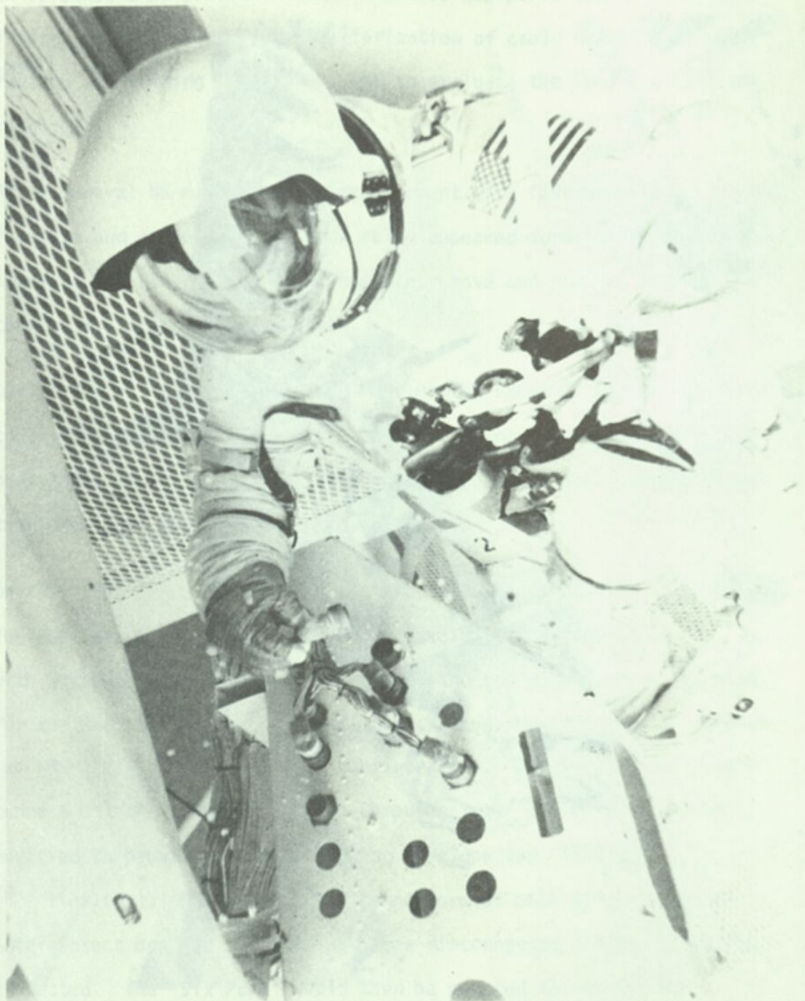
FIGURE 5-41 NBS ELECTRICAL CONNECTOR PANEL AT UPPER DA FOR RATE GYRO REPAIR
