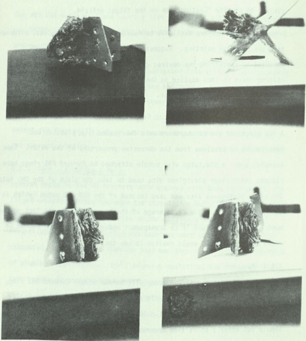
FIGURE 4-1 TM673 ALUMINUM FITTING EXFOLIATION
