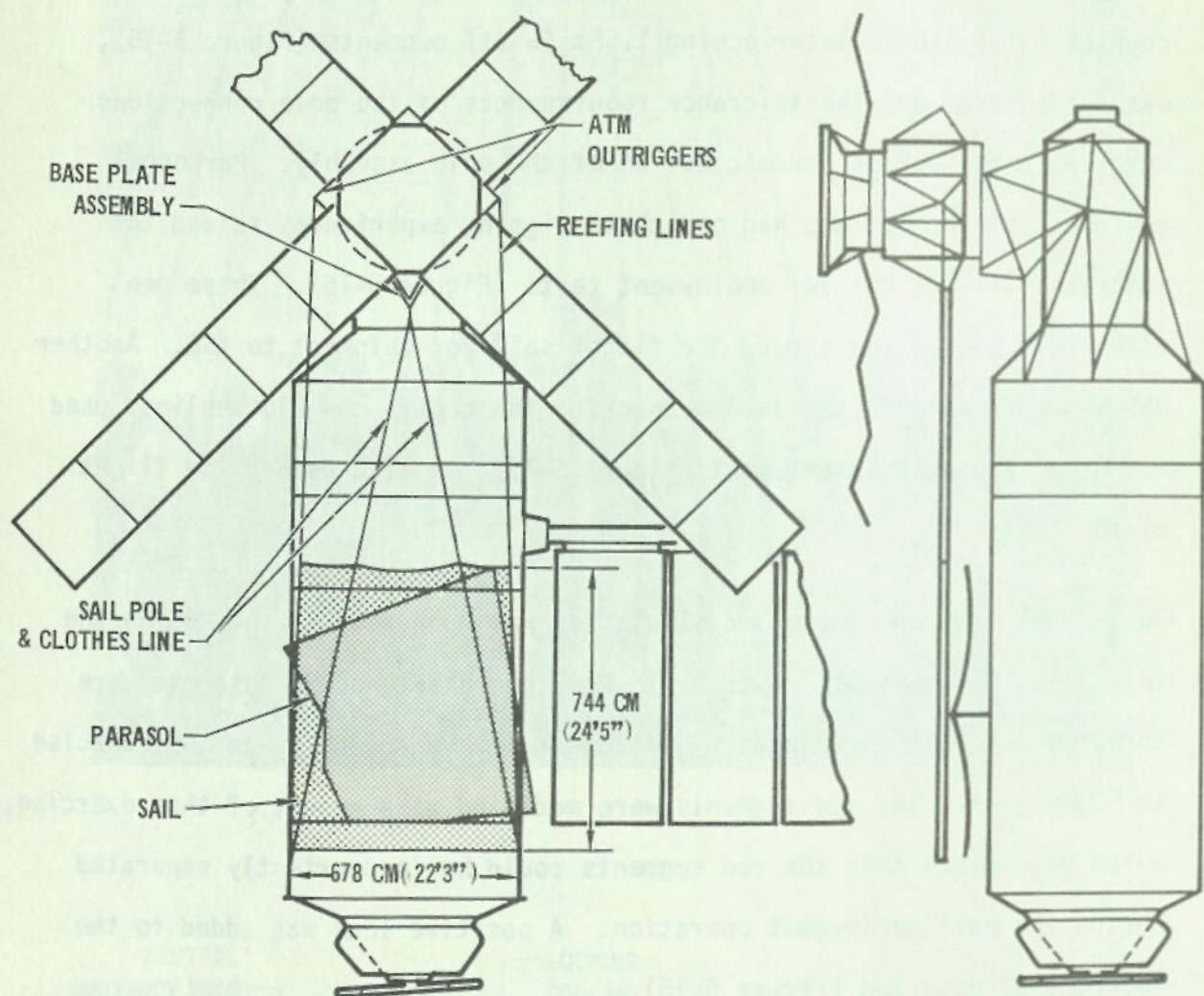
FIGURE 5-14 THERMAL SHIELD DEPLOYMENT CONFIGURATION "TWIN-POLE"
