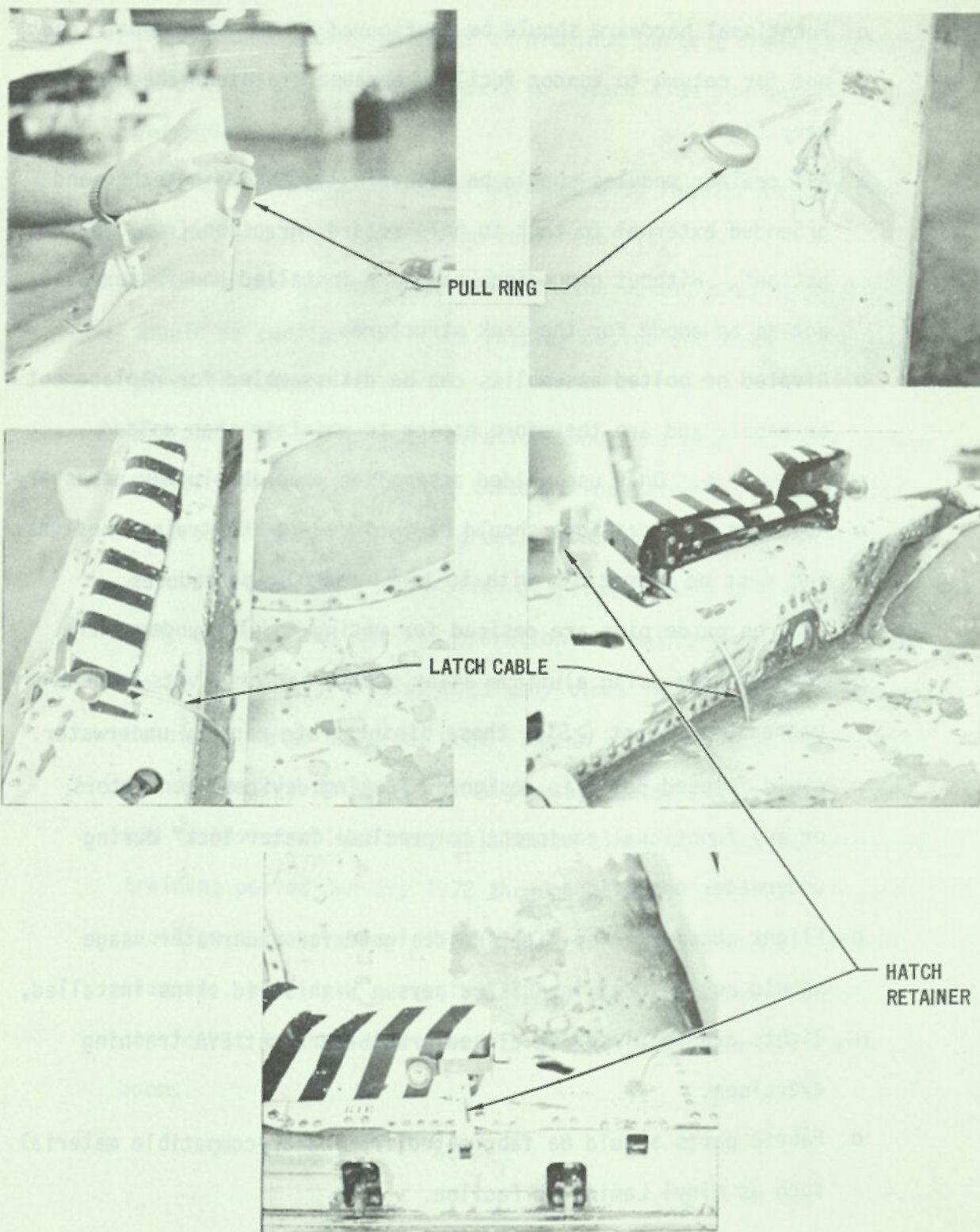
FIGURE 3-20 NBS EVA HATCH SAFETY RELREASE
