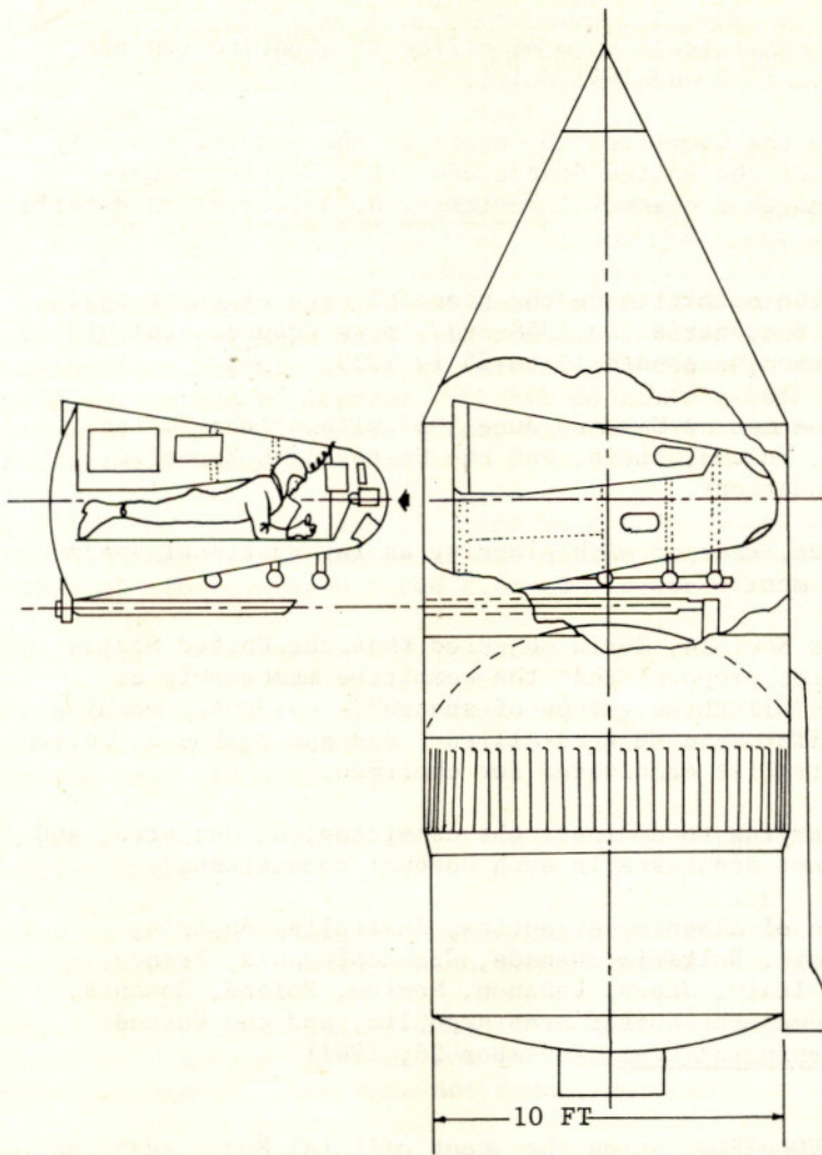
FIG. 1. Possible Configuration of Vostok 1
