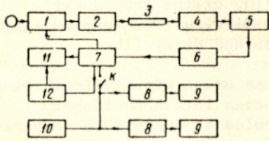
FIG. 4. Installation Block Diagram
