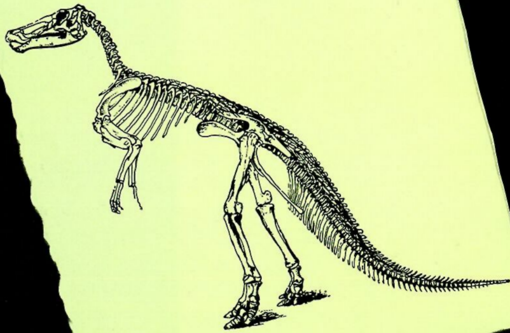
dinosaur (dī'né sôr). A group of extinct reptiles. This skeleton of a Cretaceous duck-billed dinosaur is a close relative of Hadrosaurus .
