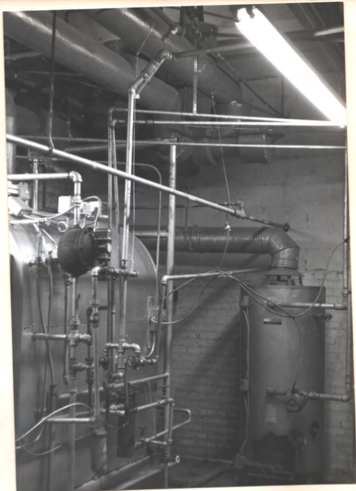
BOILER ROOM
