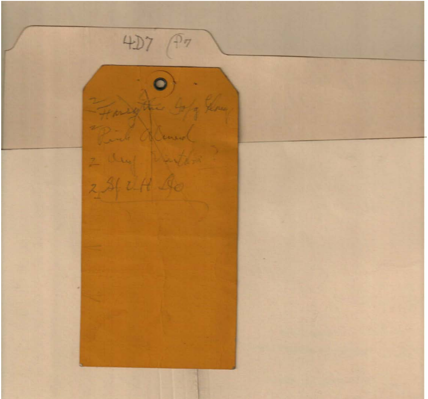
Types: label
