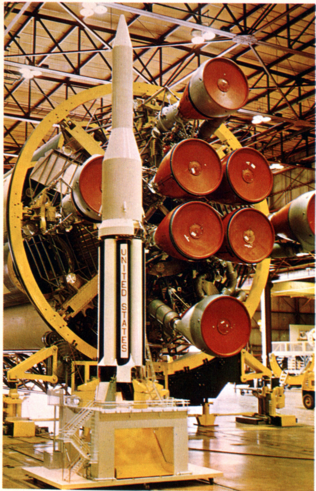
Model of Saturn Space Vehicle & "Real" Saturn Booster
